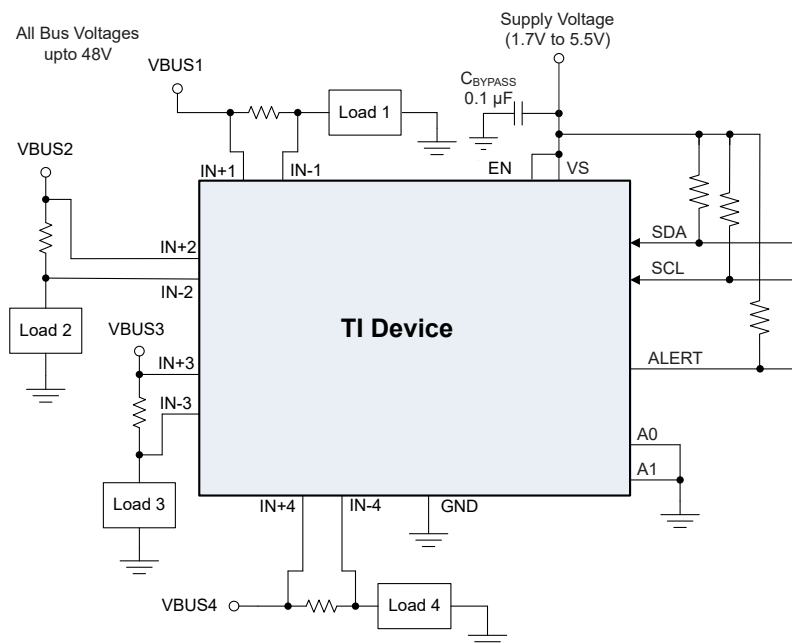
Figure 8-1. Typical High-Side Sensing Circuit Configuration, INA4230
