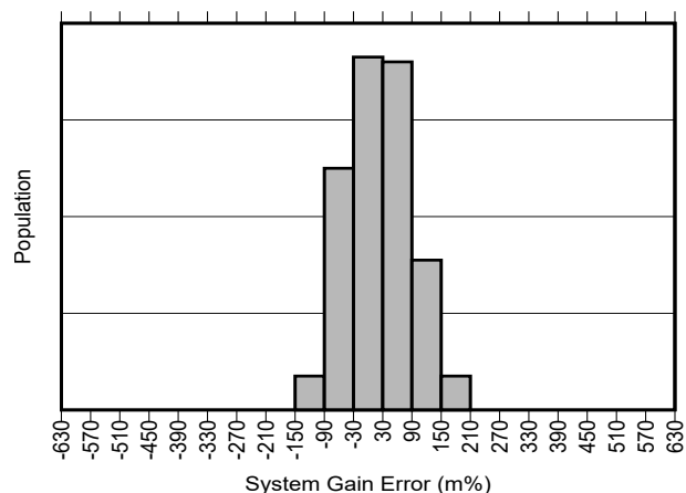
Figure 5-12. INA750B Gain Error Production Distribution
