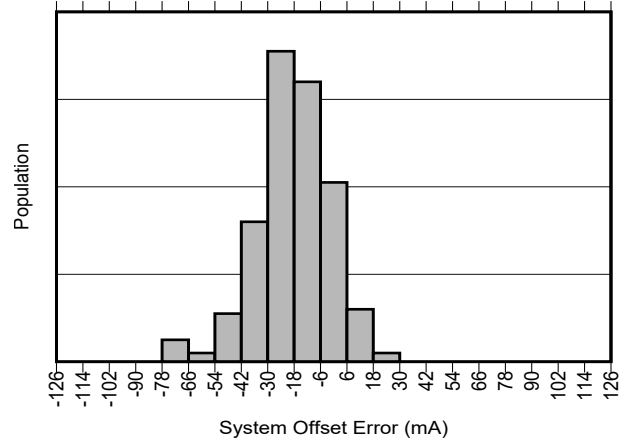
Figure 5-2. INA750B Input Offset Current Production Distribution
