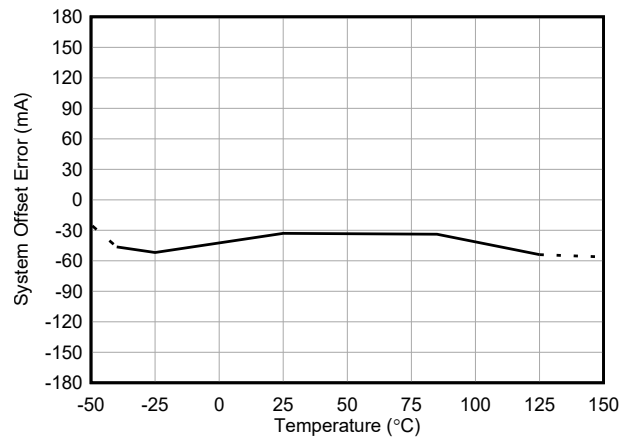
Figure 5-4. INA750B Input Offset Current vs Temperature
