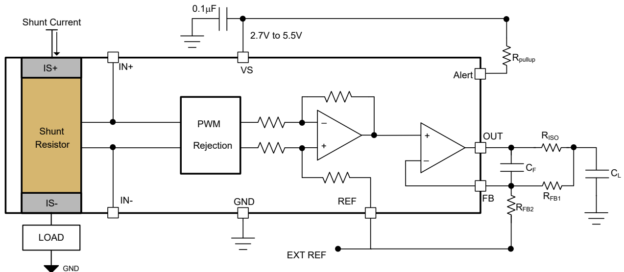
Figure 7-5. INA750x With RISO-Dual-Feedback
