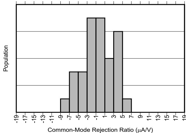
Figure 5-5. INA750A Common-Mode Rejection Production Distribution
