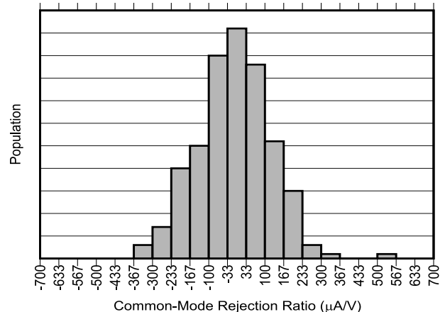
Figure 5-6. INA750B Common-Mode Rejection Production Distribution
