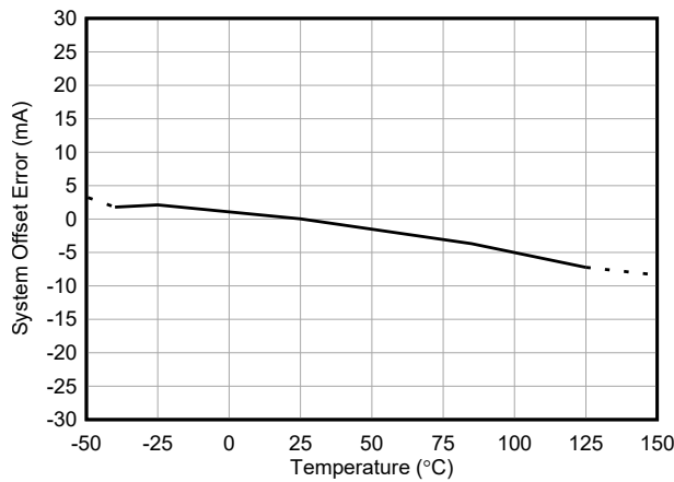
Figure 5-3. INA750A Input Offset Current vs Temperature
