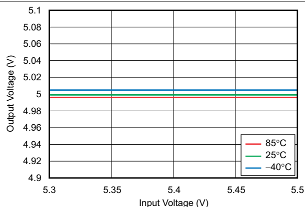
Figure 6-4. Line Regulation
