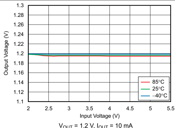
Figure 6-4. Line Regulation
