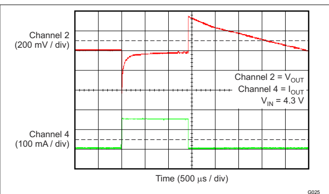
Figure 6-26. TPS70933 Load Transient (1 mA to 150 mA)
