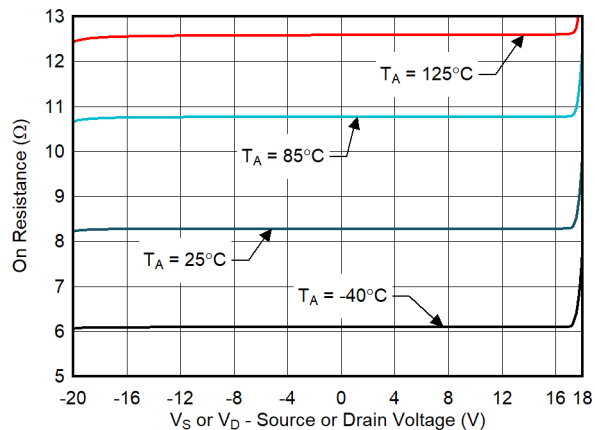
±20 V Supply Flatest Ron Region
