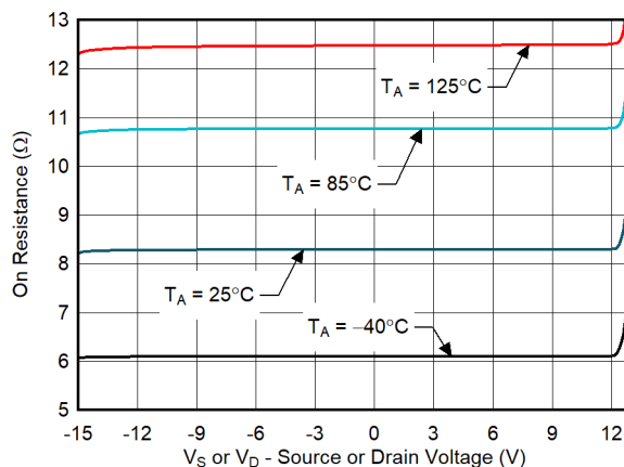
±15 V Supply Flatest Ron Region
