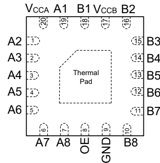
Figure 4-2. DQS Package (Top View)
