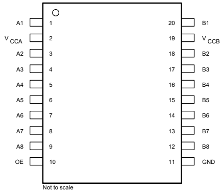
Figure 4-1. DGS/PW Package (Top View)
