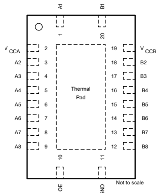
Figure 4-3. RGY/RKS Package (Top View)
