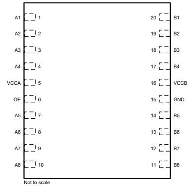
Figure 4-2. DQS Package (Top View)
