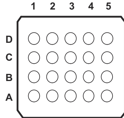
Figure 4-6. NME/GXY/ZXY PACKAGE (BOTTOM VIEW)
