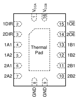
Figure 4-2. BQB Package 16-Pin WQFN (Transparent Top View)
