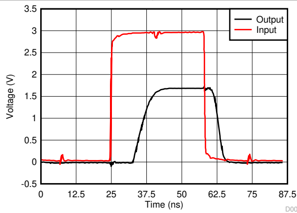
Figure 6-3. Switching Characteristics at 15 MHz Excellent Signal Integrity D003
