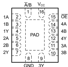
Figure 5-2. WBQB Package, 16-Pin WQFN (Transparent Top View)
