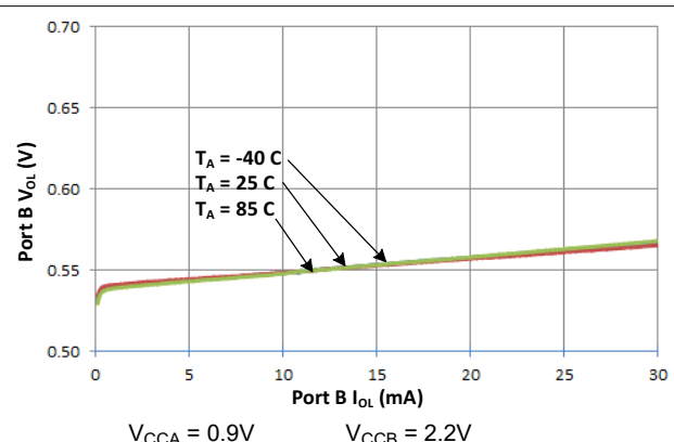
Figure 5-2. Port B V_{OL} vs I_{OL}
