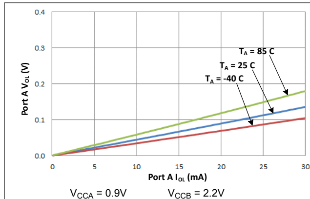
Figure 5-1. Port A V_{OL} vs I_{OL}
