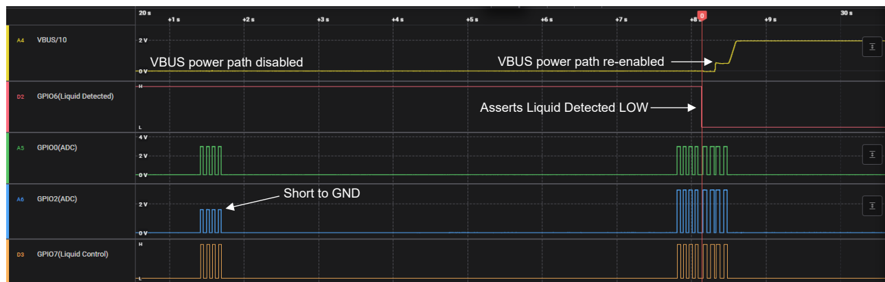
Figure 3-7. Exiting Liquid Detection Waveform
