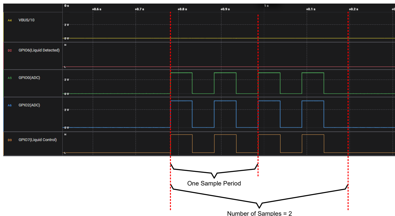
Figure 3-1. Number of Samples Waveform
