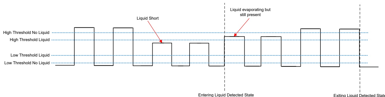
Figure 2-5. Differentiating the High Thresholds for Liquid Detection
