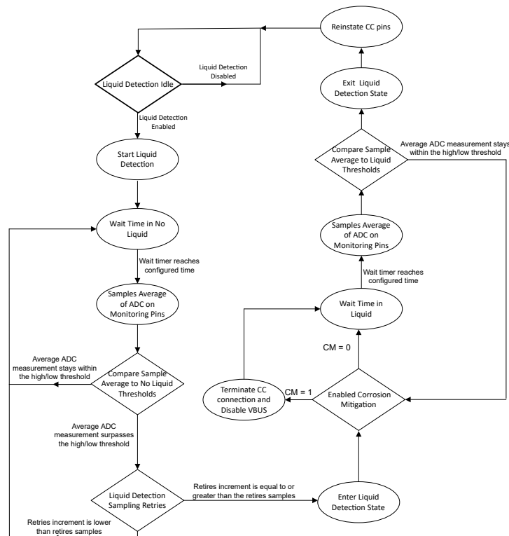
Figure 1-3. SBU Pin/Unused Pins Flow Diagram
