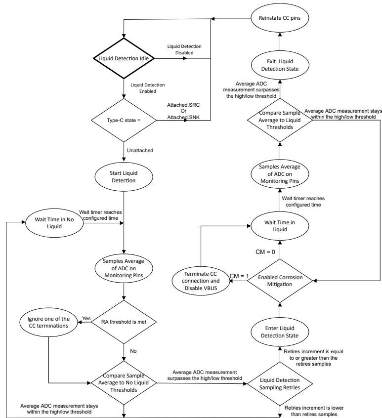
Figure 1-2. CC Pins Flow Diagram
