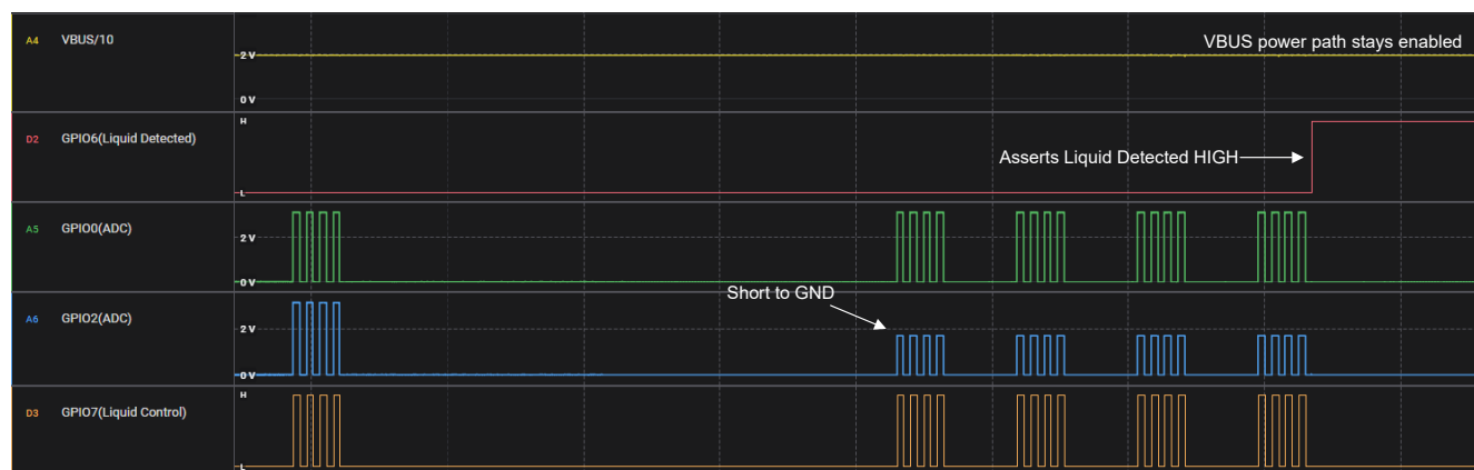
Figure 3-8. Corrosion Mitigation Disabled Waveform
