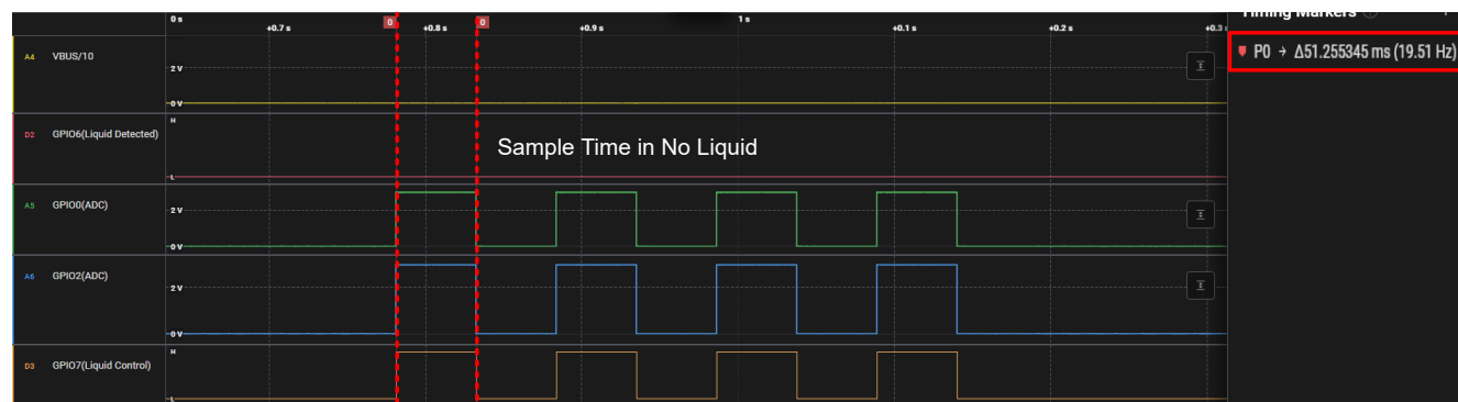
Figure 3-2. Sample Time in No Liquid Waveform
