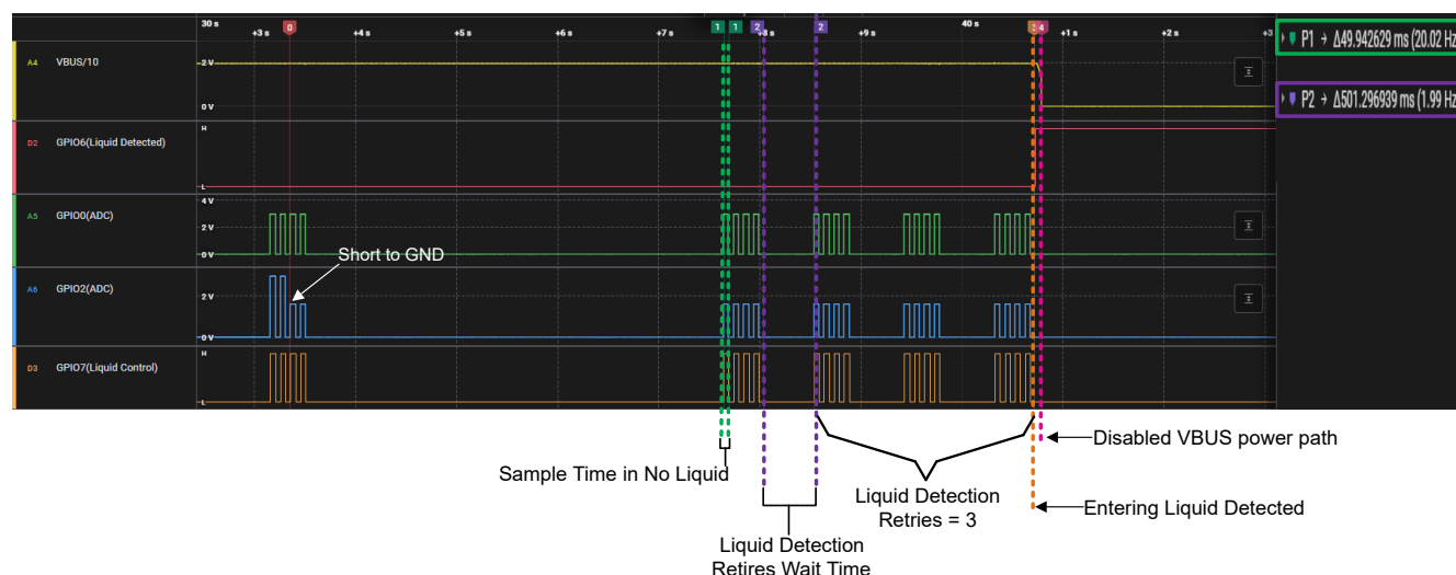
Figure 3-6. Entering Liquid Detection Waveform
