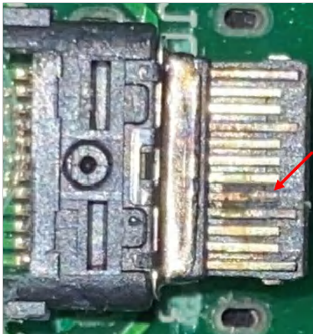
Figure 1-1. Corrosion on Type-C Port
