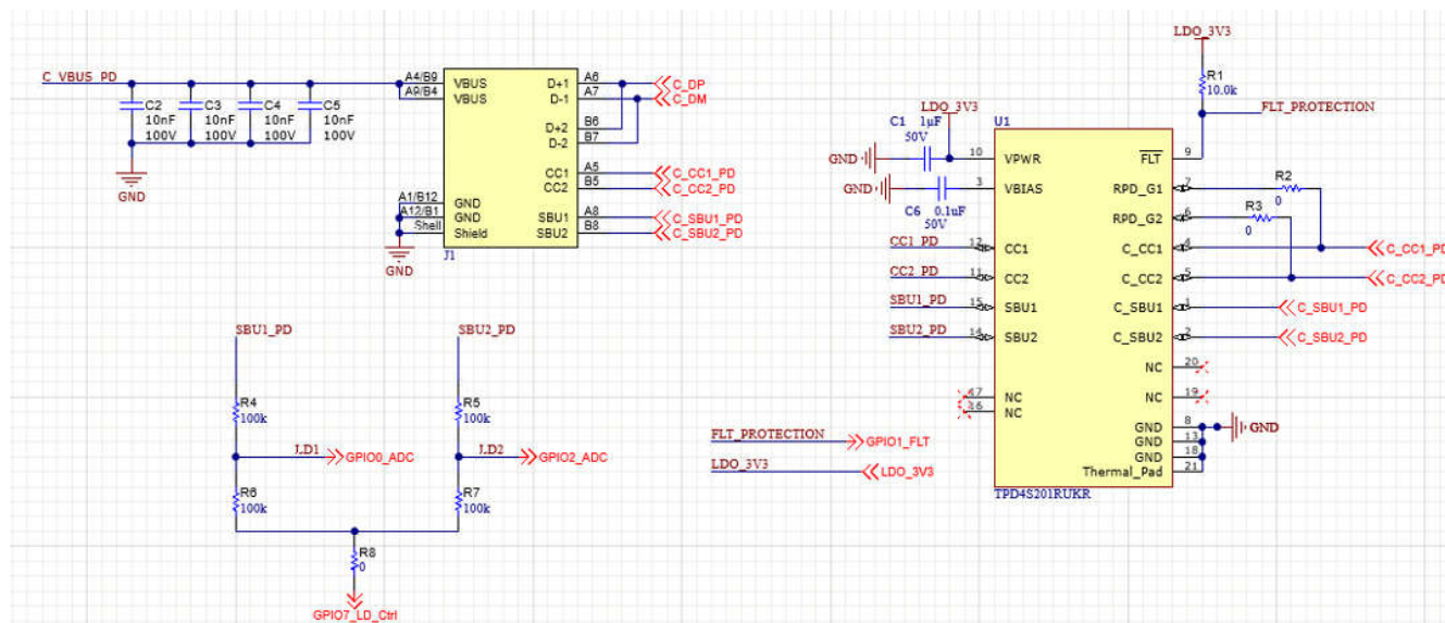
Figure 2-2. Liquid Detection Example Schematic with TPS25751A and TPD4S201
