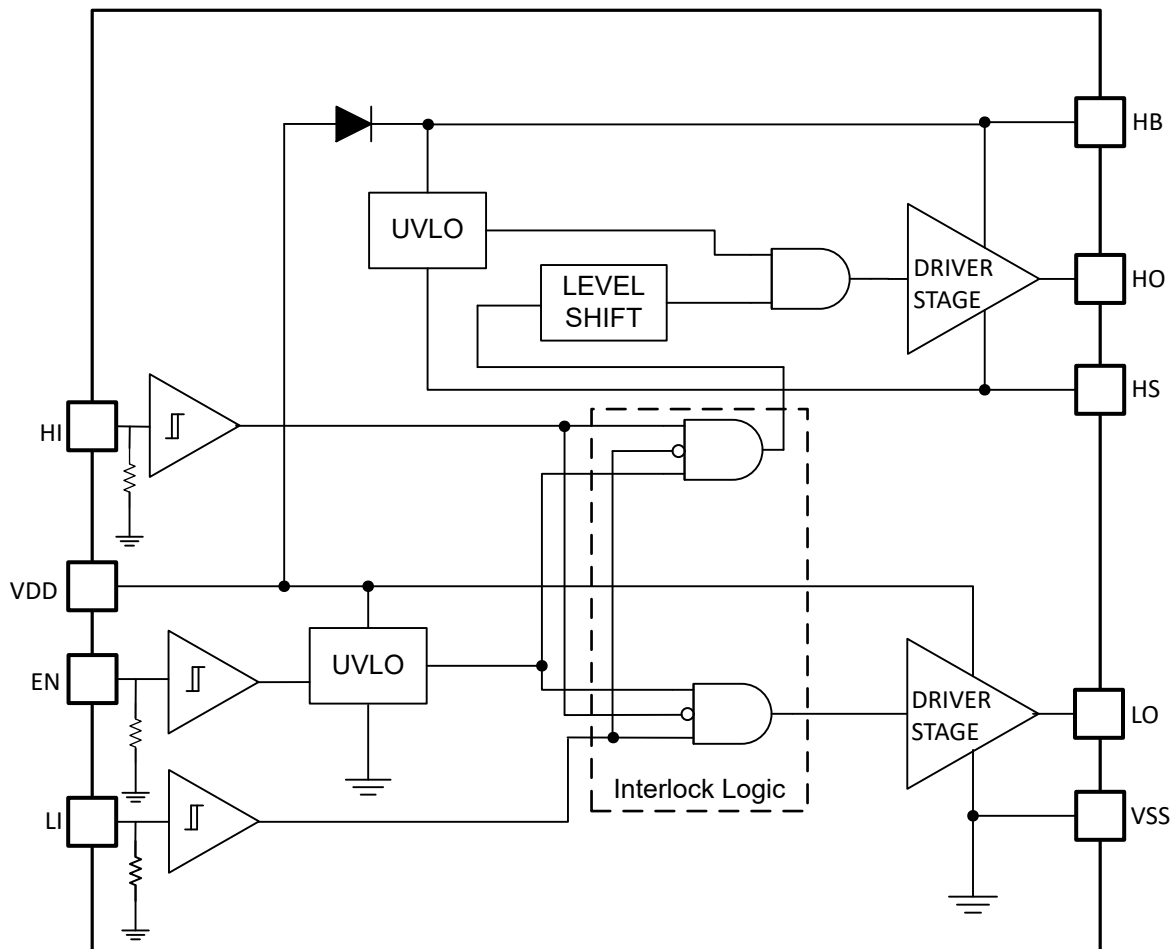
Figure 1-3. Functional Block Diagram of UCC27302A-Q1
