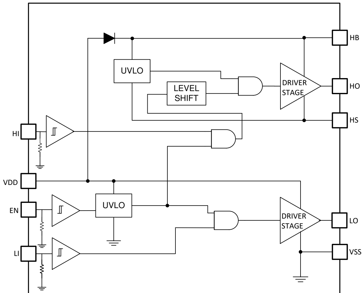
Figure 1-2. Functional Block Diagram of UCC27311A-Q1
