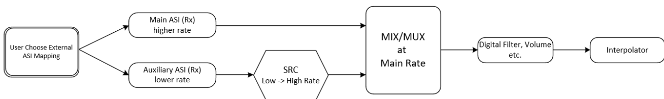
Figure 3-2. TA5x1x DAC SRC Overview - Default Mode
