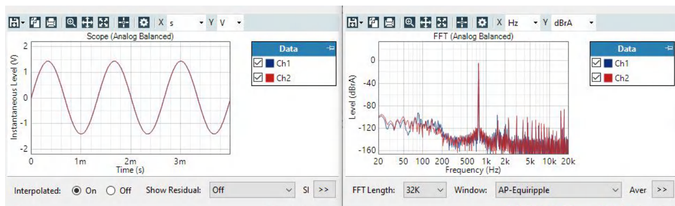
Figure 3-5. Speaker Output
