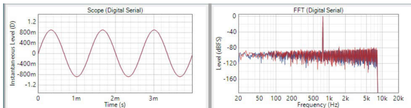
Figure 3-11. PASI ADC Output
