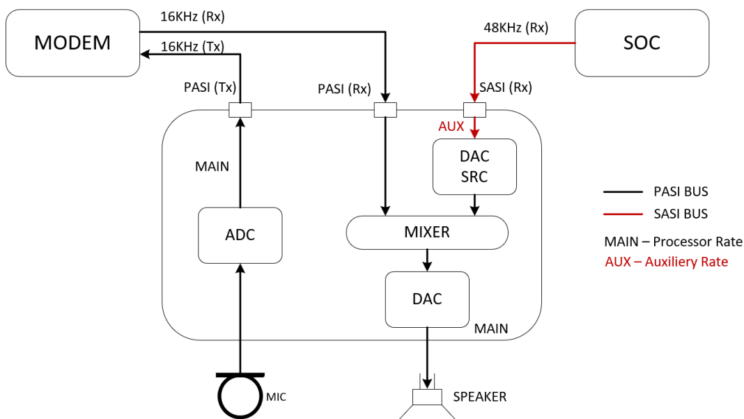
Figure 3-10. Custom Mode diagram
