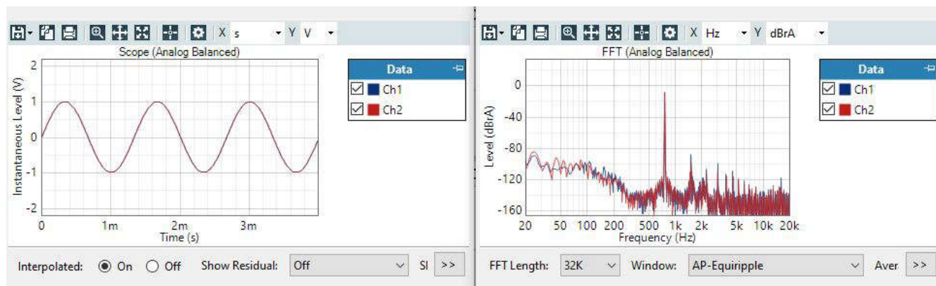
Figure 3-16. Speaker Output
