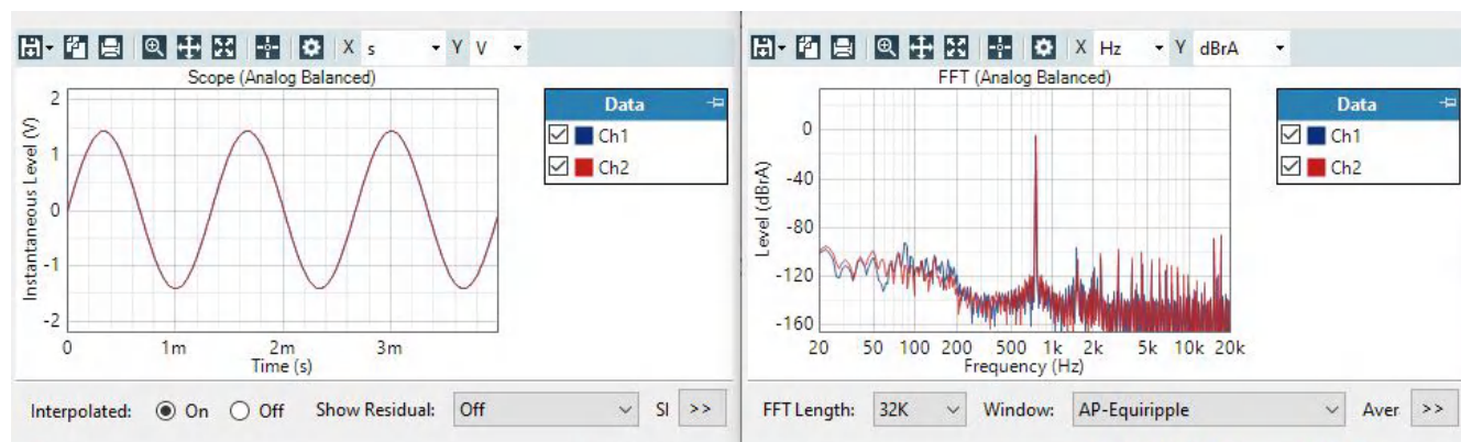
Figure 3-9. Speaker Output
