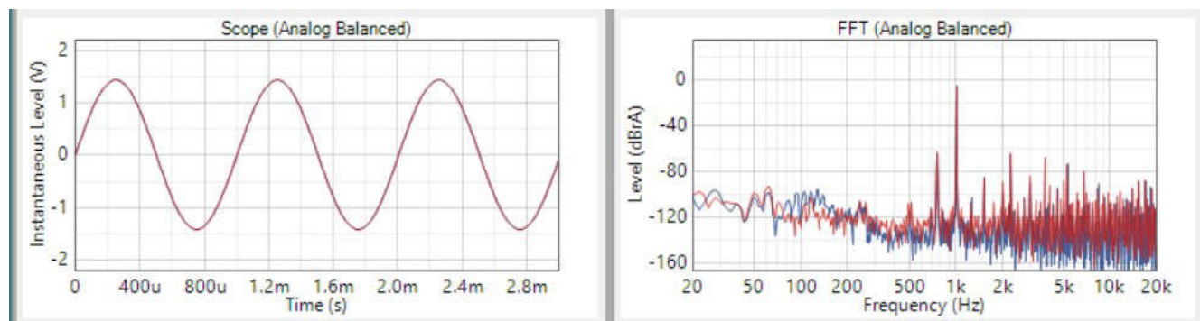
Figure 3-12. Speaker Output
