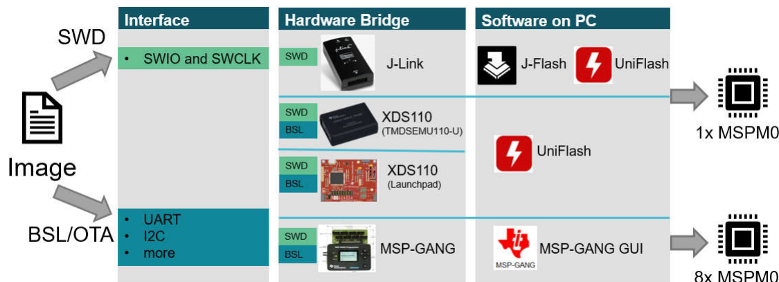
Figure 2-38. Program Software and Tool
