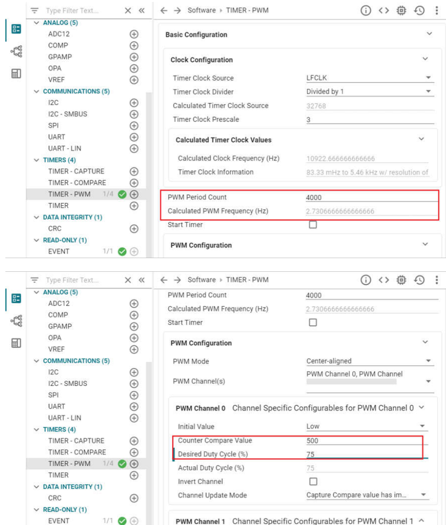
Figure 2-40. PWM Configuration in SysConfig
