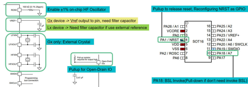
Figure 2-36. MSPM0 Minimum System Attention
