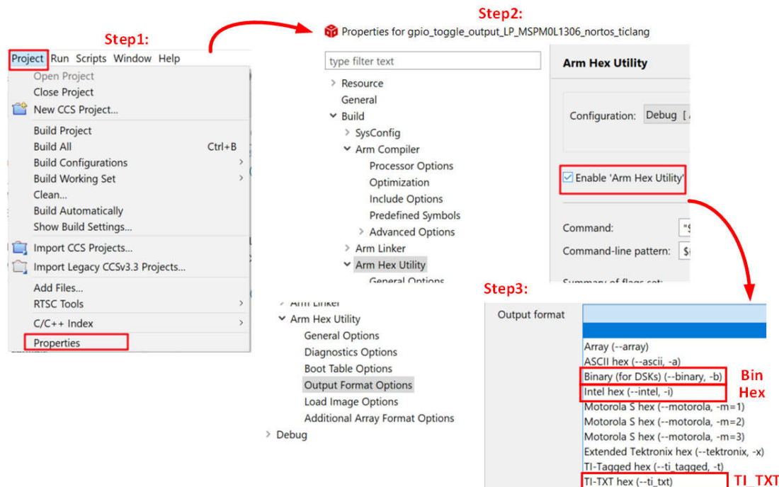
Figure 2-37. Create Program Files
