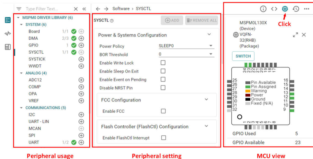
Figure 2-3. MSPM0 SysConfig
