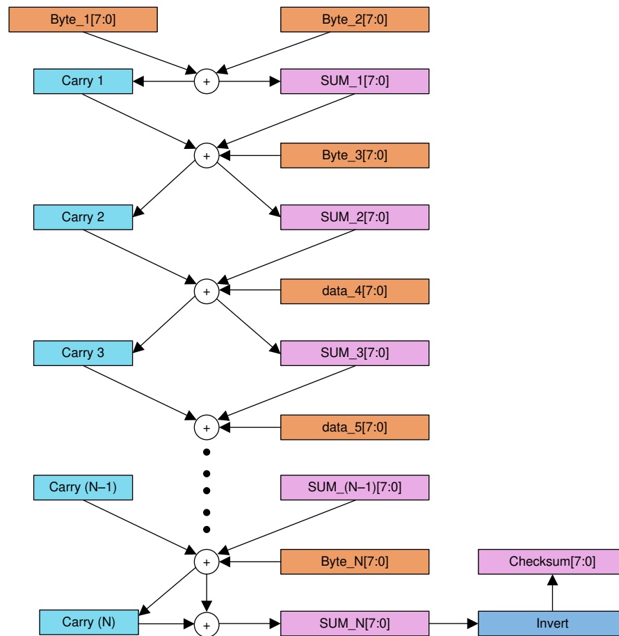
Figure 7-17. Checksum Calculation
