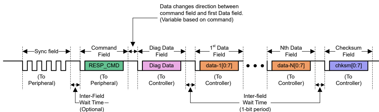
Figure 7-25. UART Response Example
