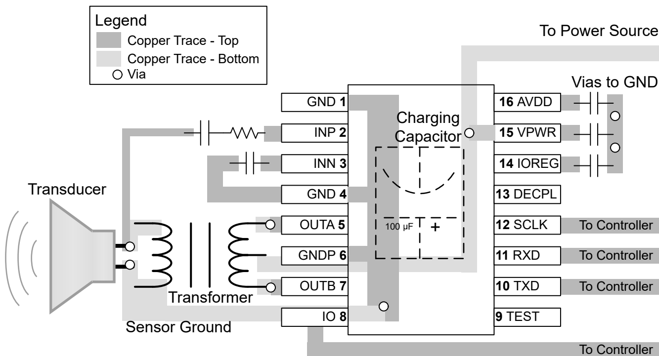
Figure 8-9. PGA460 Layout Example
