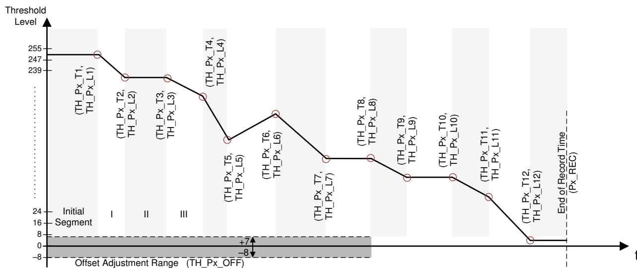
Figure 7-6. Threshold Assignment Example
