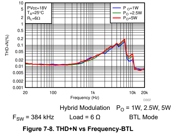
Figure 7-8. THD+N vs Frequency-BTL
