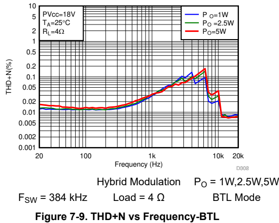
Figure 7-9. THD+N vs Frequency-BTL
