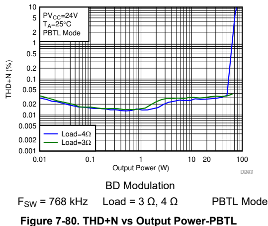
Figure 7-80. THD+N vs Output Power-PBTL
