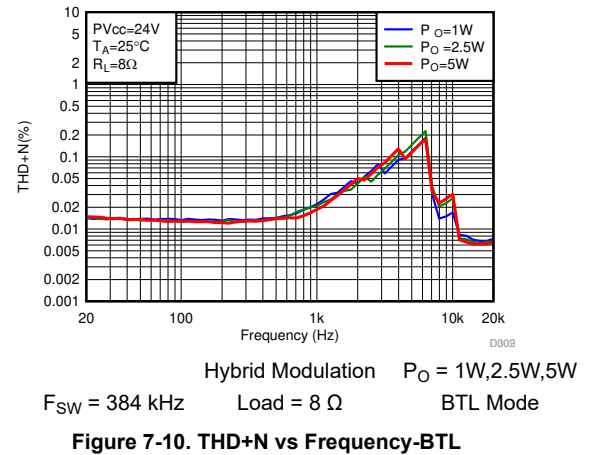
Figure 7-10. THD+N vs Frequency-BTL
