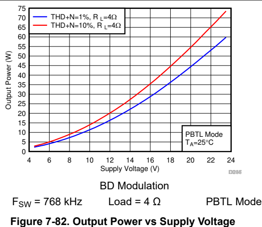
Figure 7-82. Output Power vs Supply Voltage
