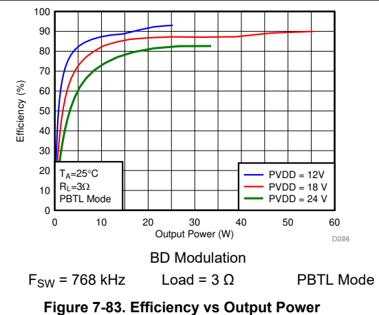
Figure 7-83. Efficiency vs Output Power
