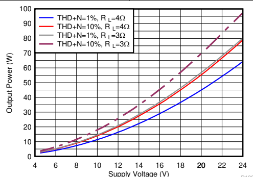
Hybrid Modulation F SW = 384 kHz Load = 3 Ω, 4 Ω PBTL Mode
