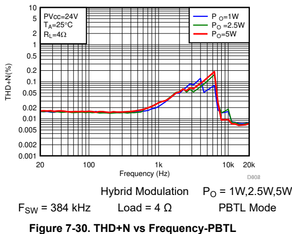
Figure 7-30. THD+N vs Frequency-PBTL
