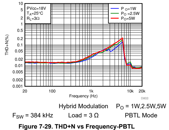
Figure 7-29. THD+N vs Frequency-PBTL
