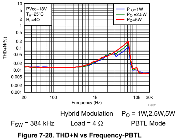
Figure 7-28. THD+N vs Frequency-PBTL
