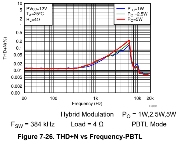
Figure 7-26. THD+N vs Frequency-PBTL
