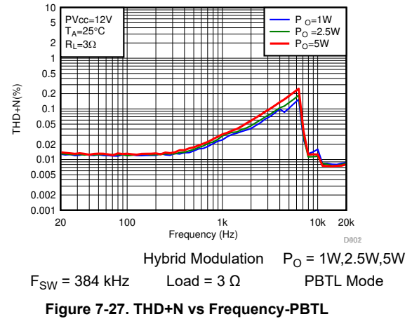
Figure 7-27. THD+N vs Frequency-PBTL
