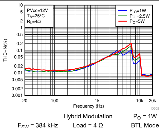
Figure 7-6. THD+N vs Frequency-BTL
