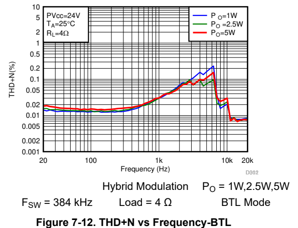
Figure 7-12. THD+N vs Frequency-BTL
