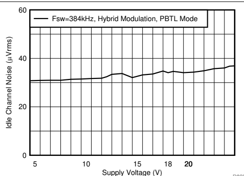
Hybrid Modulation F SW = 384 kHz Load = 6 Ω PBTL Mode Figure 7-39. Idle Channel Noise vs Supply Voltage
