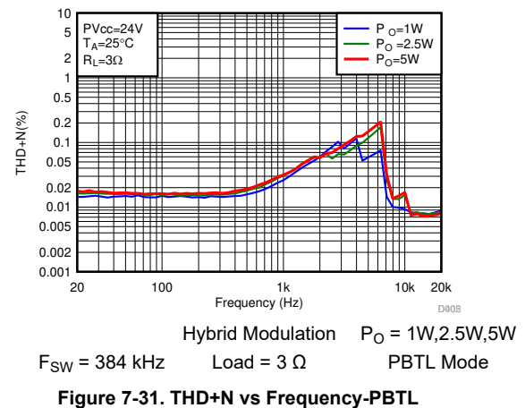
Figure 7-31. THD+N vs Frequency-PBTL
