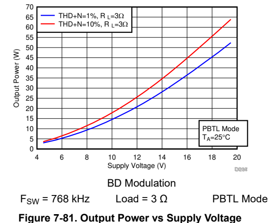
Figure 7-81. Output Power vs Supply Voltage
