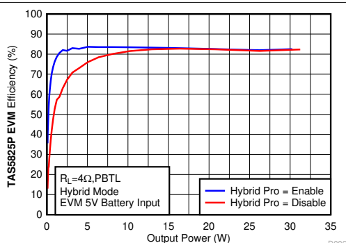
Hybrid Modulation F SW = 384 kHz 5 V Battery Input Default PPC3 Setting Load=4Ω, PBTL approximately 5 V – (-5.5dB AGAIN) 16 V Boost
