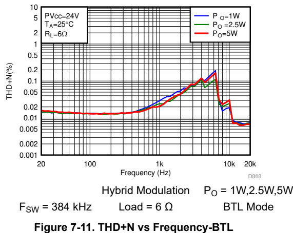
Figure 7-11. THD+N vs Frequency-BTL
