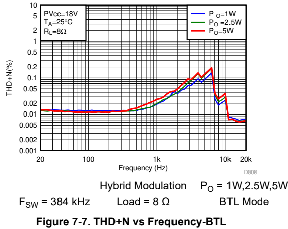
Figure 7-7. THD+N vs Frequency-BTL
