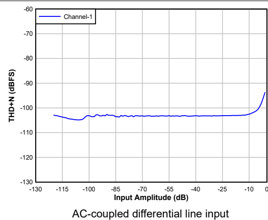
Figure 9-3. ADC THD+N Level vs Input
