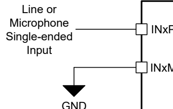
Figure 7-18. Single-ended DC-Coupled Input Connection (ADC_CHx_INSRC set to 2'b01 and ADC_CHx_CM_TOL set to 2'b01 or 2'10)
