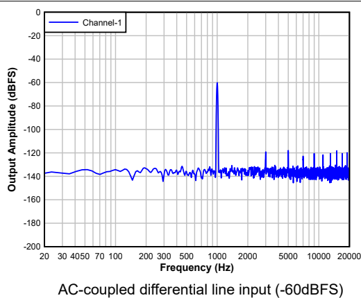
Figure 9-2. ADC FFT with -60dBFS Input
