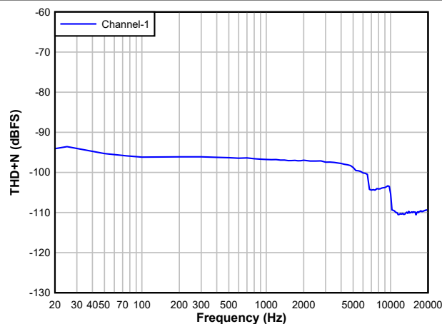
Figure 6-27. DAC THD+N Level vs Frequency
