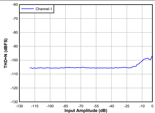
Figure 6-20. DAC THD+N Level vs Input
