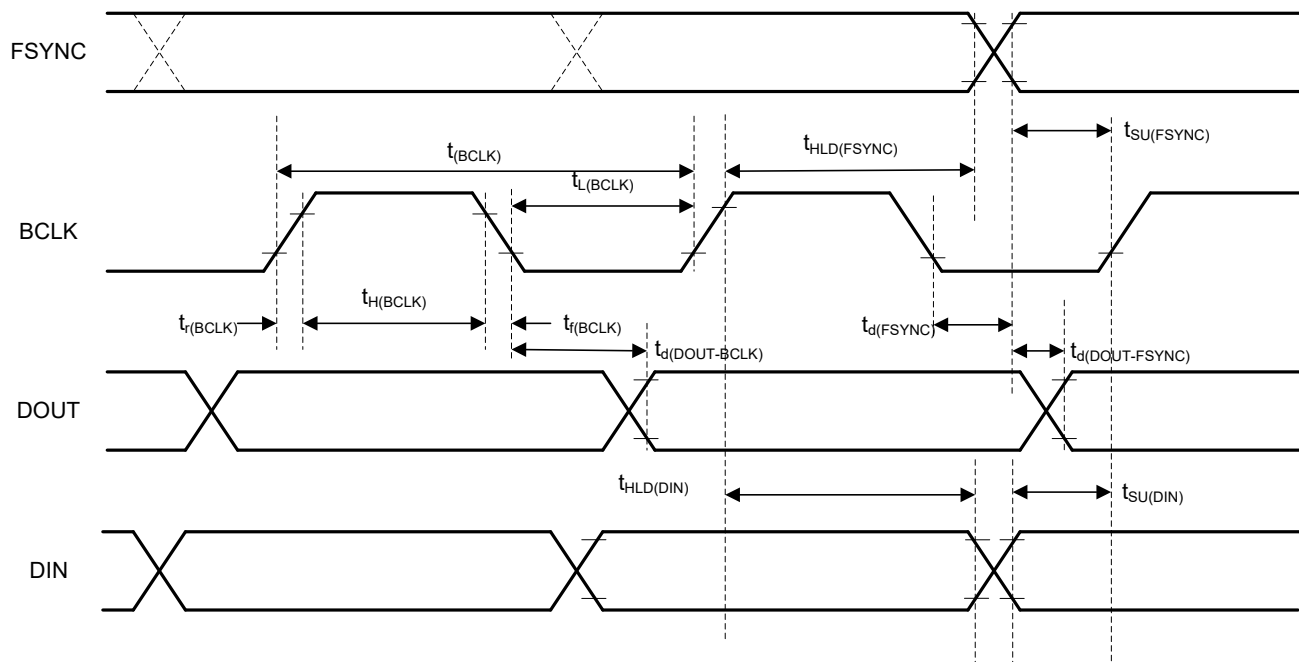
Figure 6-3. TDM (With BCLK_POL = 1), I²S, and LJ Interface Timing Diagram
