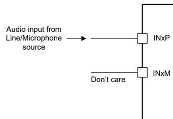
Figure 7-20. Single-ended mux on INxP DC-Coupled Input Connection (ADC_CHx_INSRC set to 2'b10 and ADC_CHx_CM_TOL set to 2'b01 or 2'10)
