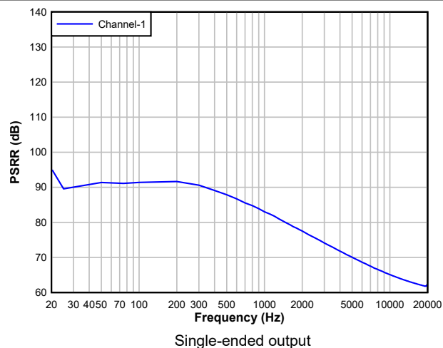
Figure 6-33. DAC PSRR vs Frequency
