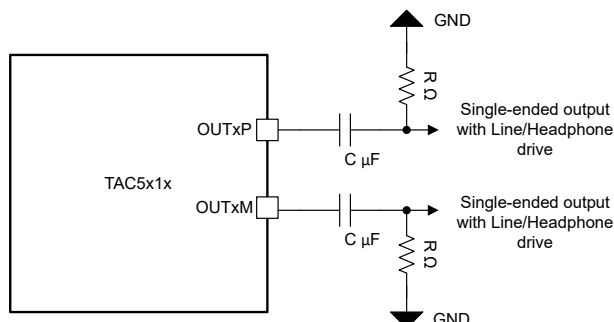
Figure 7-24. Stereo Single-ended Output Connection (OUT1x_CFG[2:0] = 3'b001)
