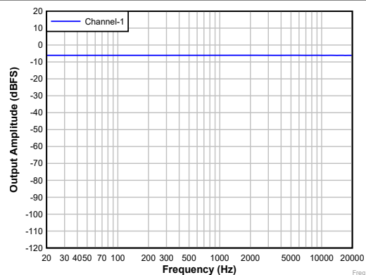
Figure 6-34. DAC Frequency Response
