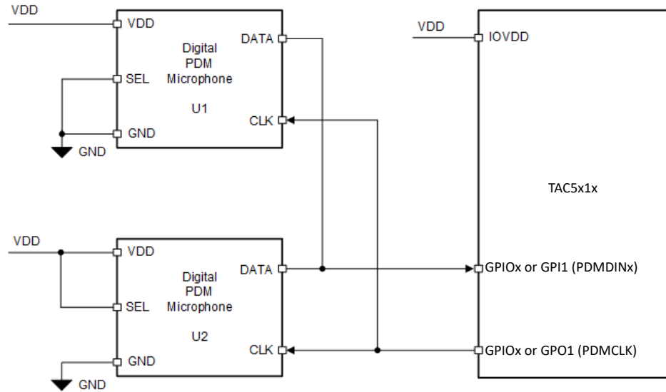
Figure 7-25. Digital PDM Microphones Connection Diagram for the TAC5111
