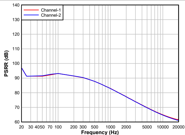
Figure 6-26. DAC PSRR vs Frequency
