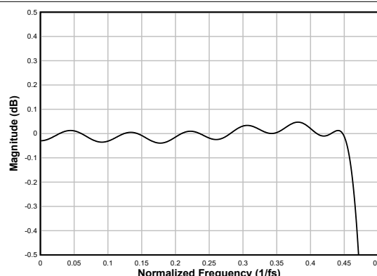
Figure 7-22. Linear-phase Decimation Filter Pass-Band Ripple
