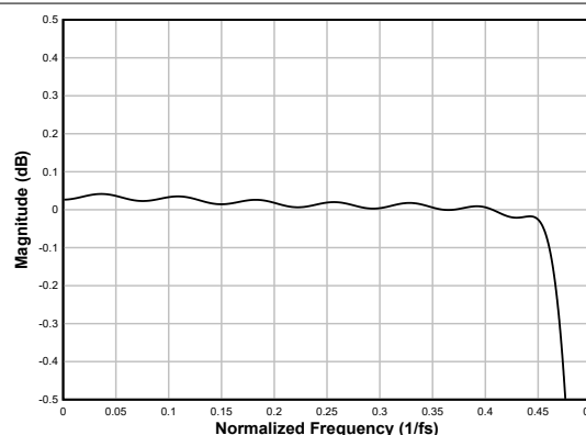
Figure 7-16. Linear-phase Decimation Filter Pass-Band Ripple
