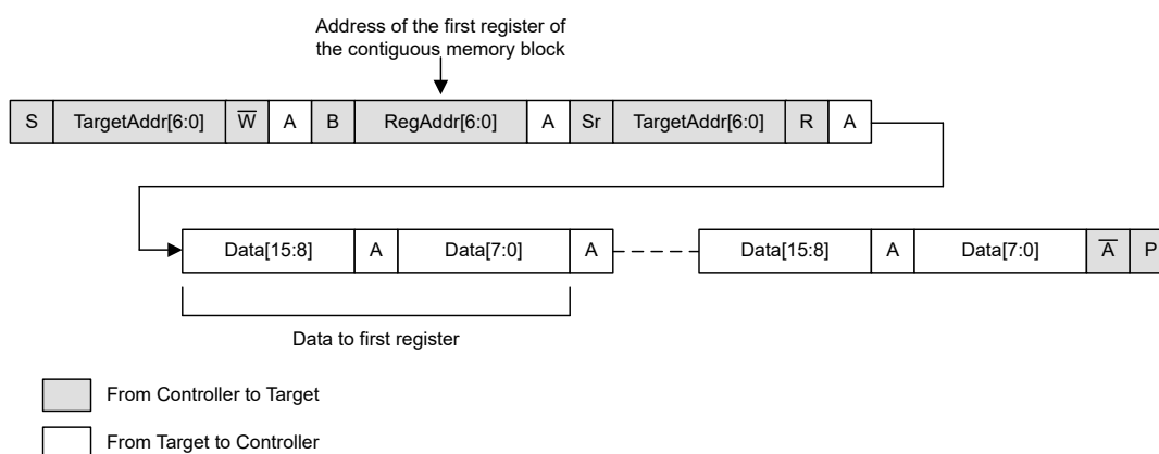
Figure 6-5. I²C Block Read Access
