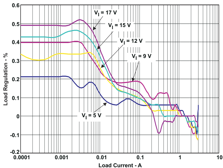
Figure 3-4. Load Regulation With 2.2- \mu\text{H} Inductor and F_{SW} = \text{LOW} (High Frequency)
