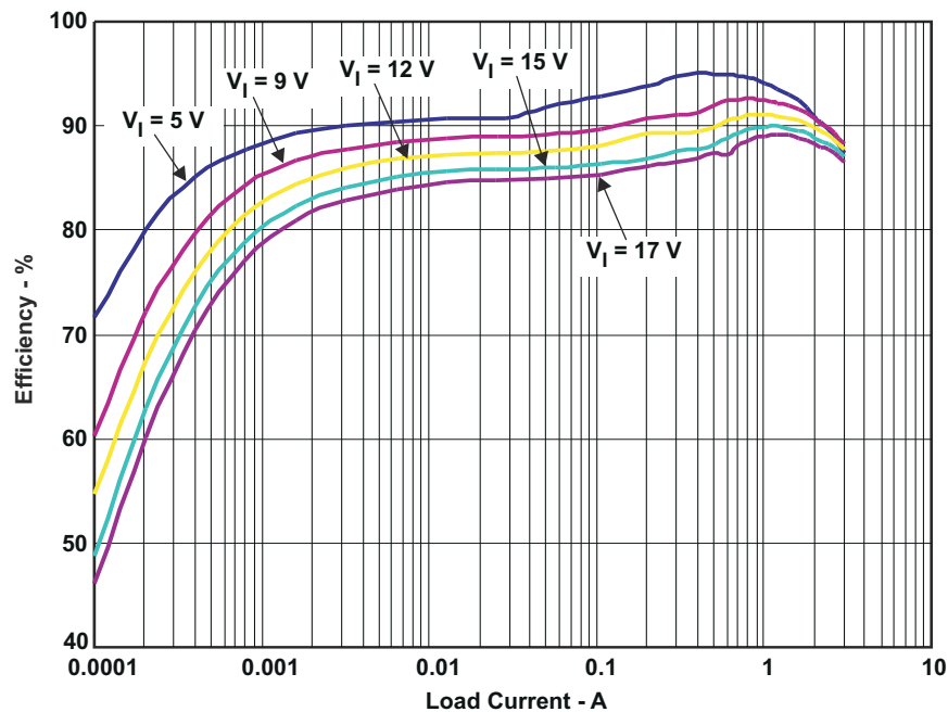
Figure 3-3. Efficiency With 2.2- \mu\text{H} Inductor and F_{SW} = \text{HIGH} (Low Frequency)
