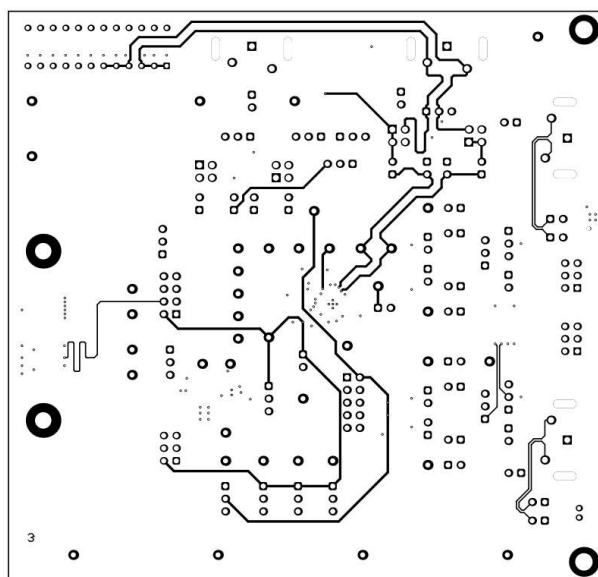
Figure 4-17. TA5x42 EVM Signal Layer 1
