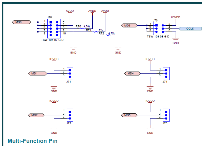
Figure 4-8. TAD5242 EVM Connectors and Supporting Circuitry Schematic
