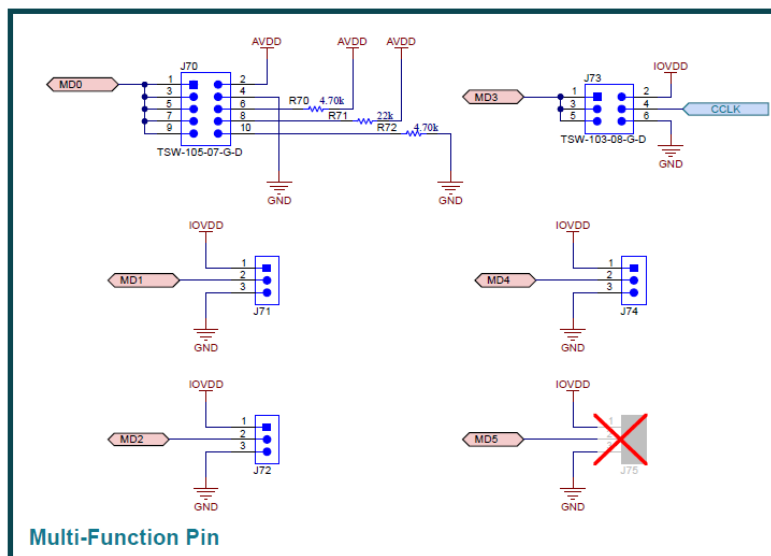
Figure 4-6. TAA5242 EVM Connectors and Supporting Circuitry Schematic
