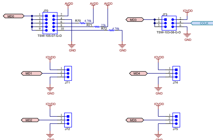
Figure 2-11. Multi-Function Pin Setting
