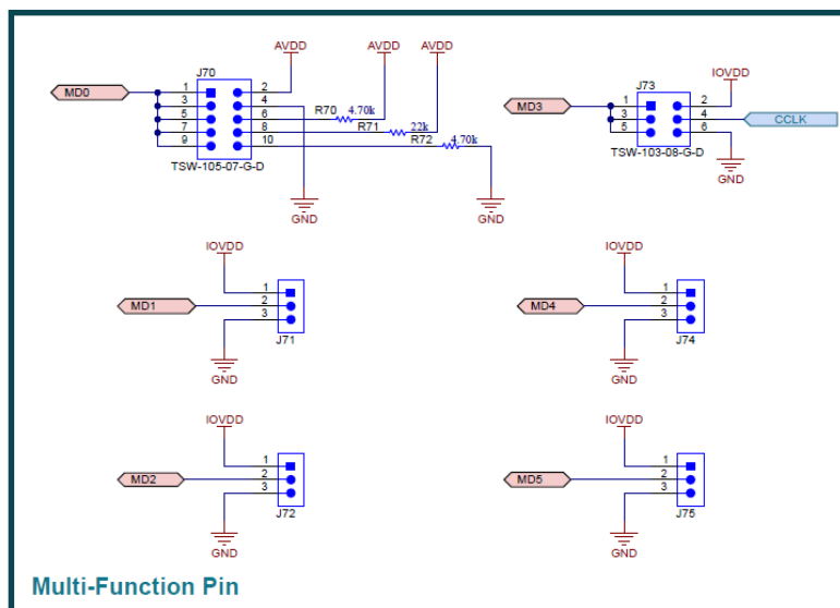
Figure 4-4. TAC5142 EVM Connectors and Supporting Circuitry Schematic
