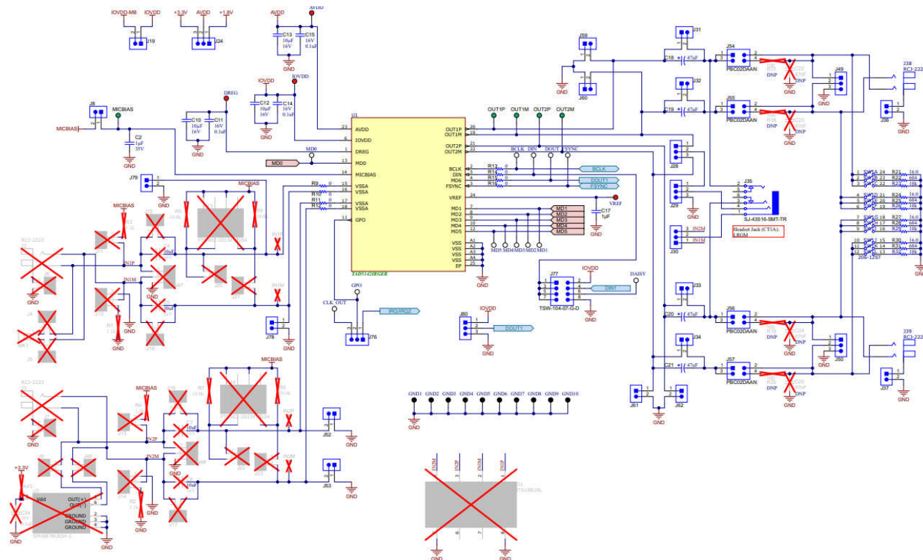
Figure 4-9. TAD5142 EVM Main DUT Schematic
