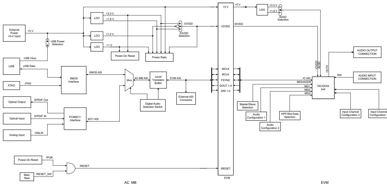
Figure 2-1. TAx5x42 EVM Block Diagram
