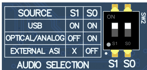
Figure 2-3. AC-MB USB Audio Setting
