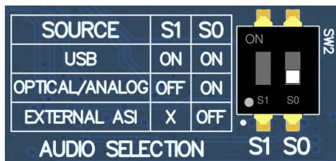
Figure 2-5. AC-MB External Audio Interface Setting
