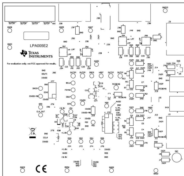
Figure 4-11. TAx5x42 EVM Top Silkscreen
