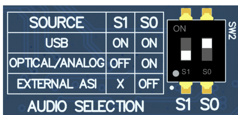
Figure 2-4. AC-MB Optical or Auxiliary Analog Audio Input Setting
