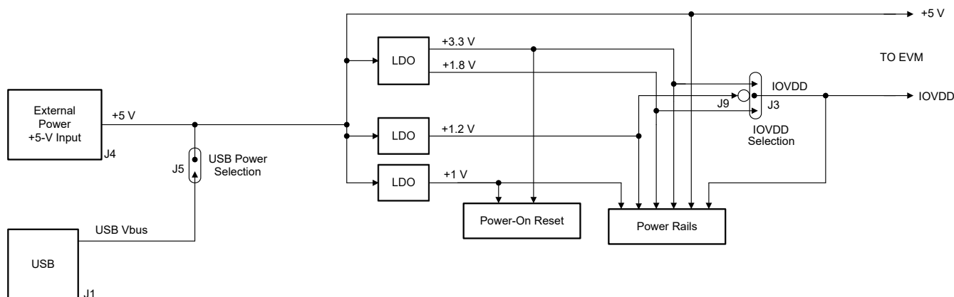
Figure 2-7. Power-Supply Distribution of the AC-MB
