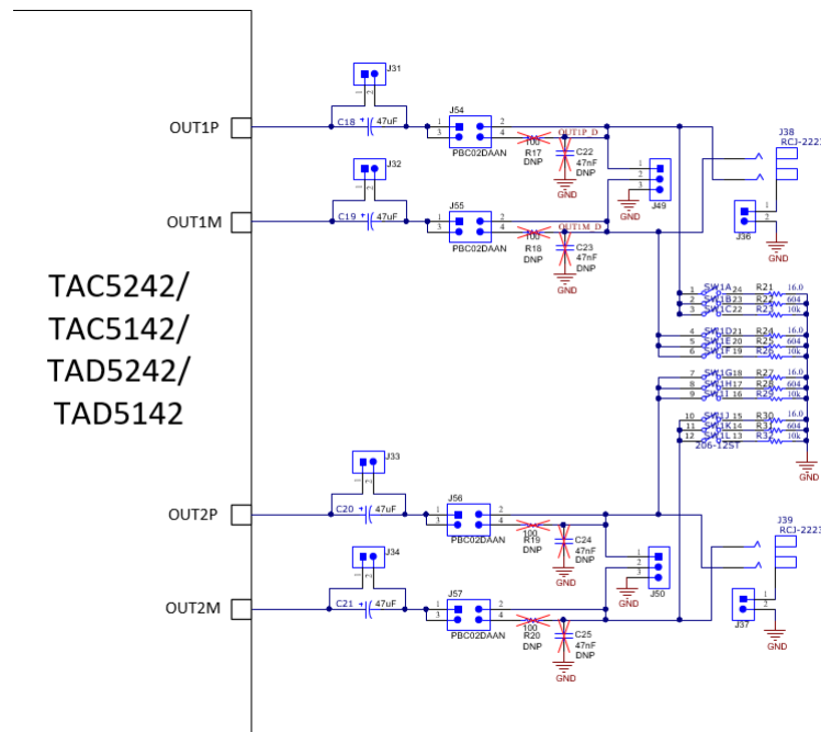
Figure 2-9. TAC5242/TAC5142/TAD5242/TAD5142 EVM Output Architecture
