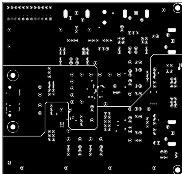
Figure 4-13. TAx5x42 EVM Power Layer 1
