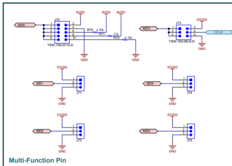
Figure 4-10. TAD5142 EVM Connectors and Supporting Circuitry Schematic
