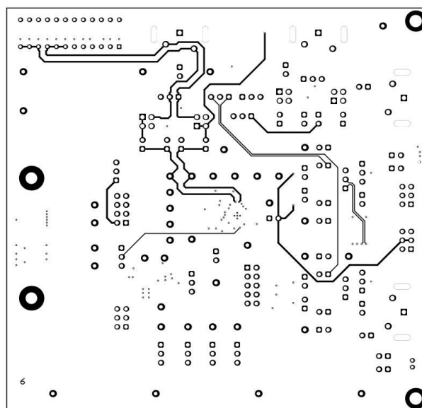
Figure 4-18. TA5x42 EVM Signal Layer 2
