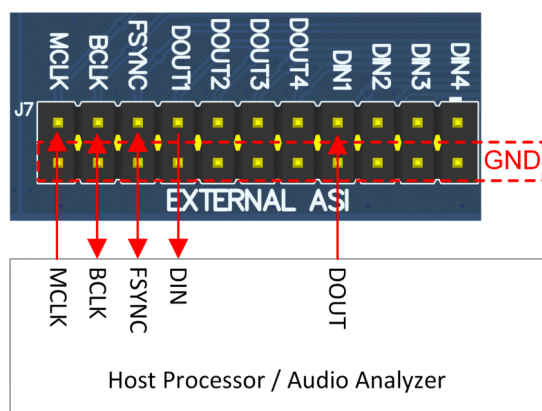
Figure 2-6. AC-MB Connection with External Audio Serial Interface
