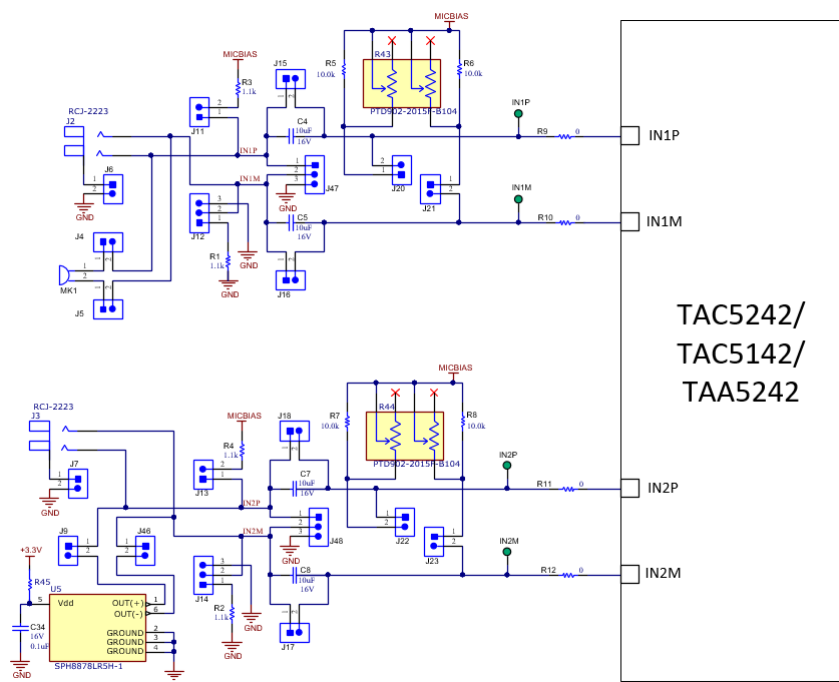
Figure 2-8. TAC5242/TAC5142/TAA5242 EVM Input Architecture for Channel 1 and 2
