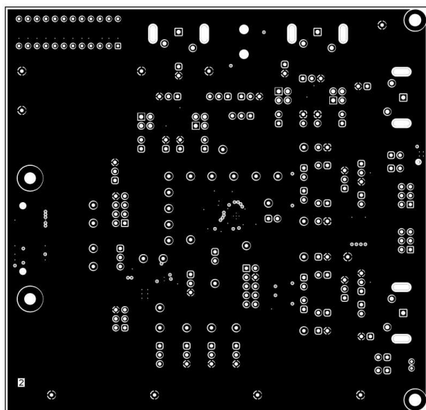
Figure 4-15. TA5x42 EVM Ground Layer 1
