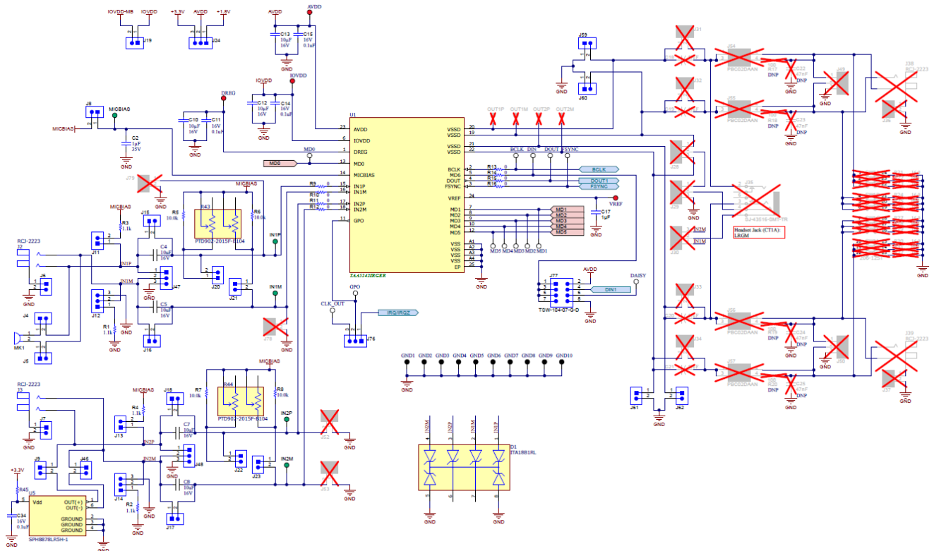
Figure 4-5. TAA5242 EVM Main DUT Schematic
