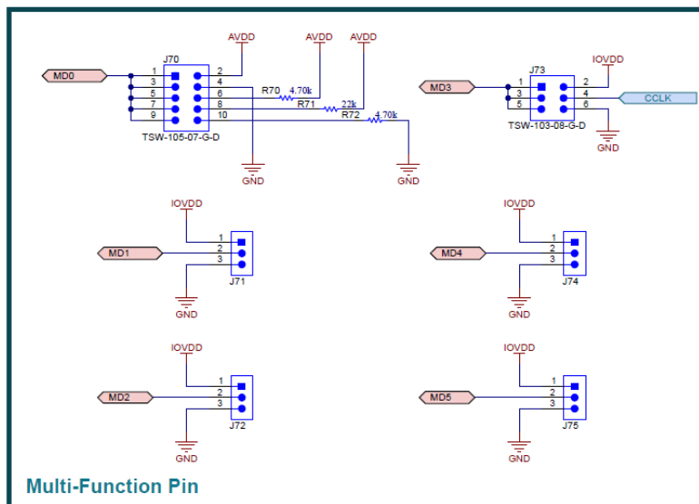
Figure 4-2. TAC5242 EVM Connectors and Supporting Circuitry Schematic
