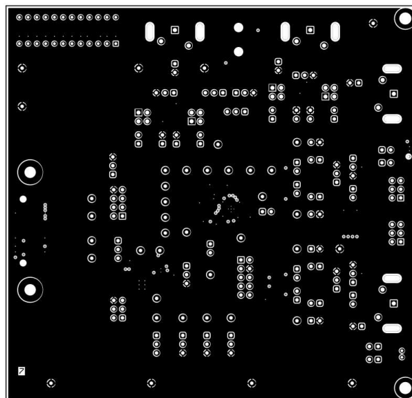
Figure 4-16. TA5x42 EVM Ground Layer 2
