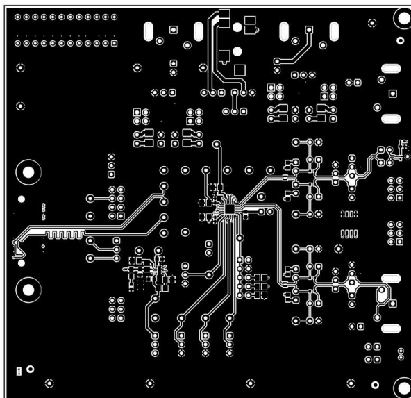
Figure 4-12. TAx5x42 EVM Top Layer
