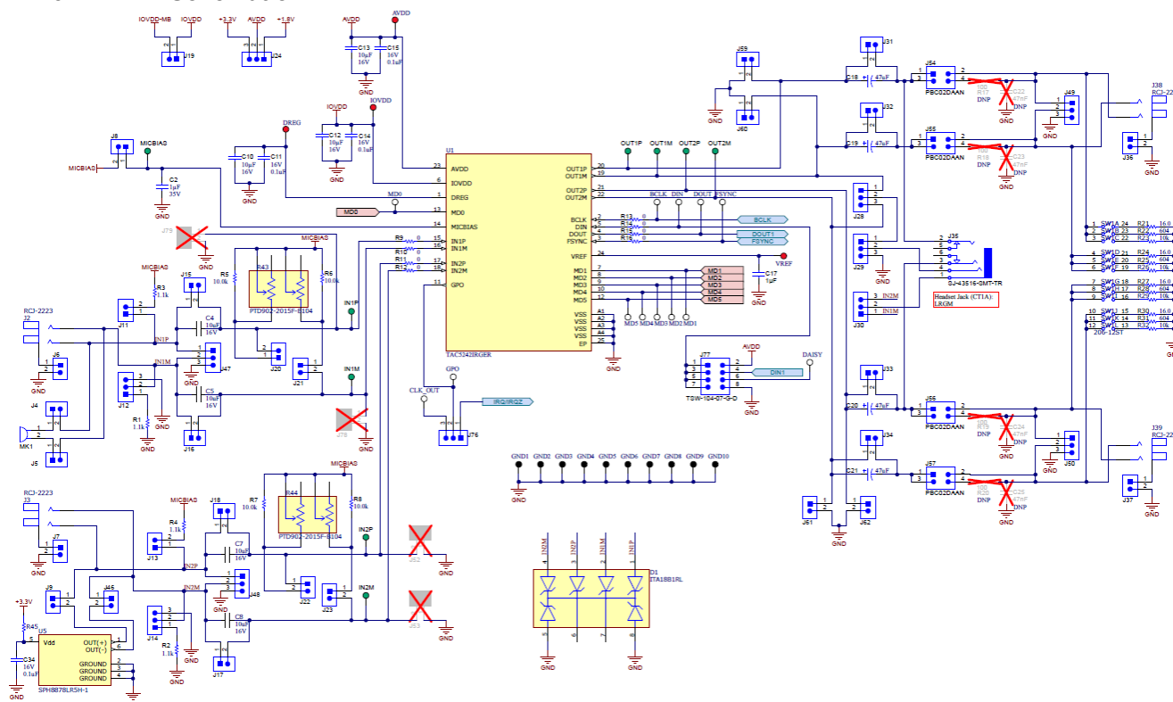
Figure 4-1. TAC5242 EVM Main DUT Schematic
