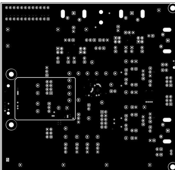
Figure 4-14. TAx5x42 EVM Power Layer 2
