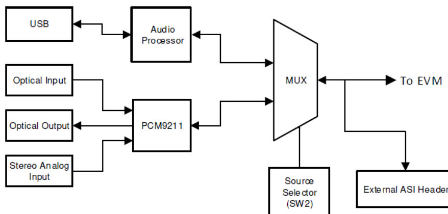
Figure 2-2. AC-MB Audio Interface Block Diagram
