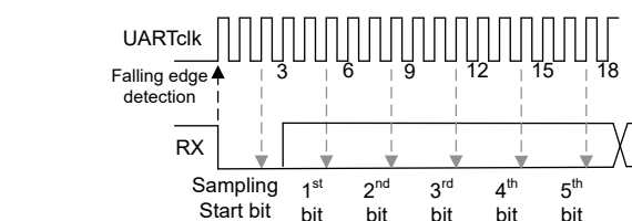
Figure 22-3. UART Oversampling mode
