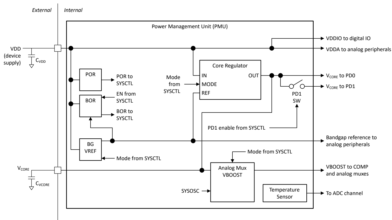
Figure 2-2. MSPM33C3 PMU Block Diagram
