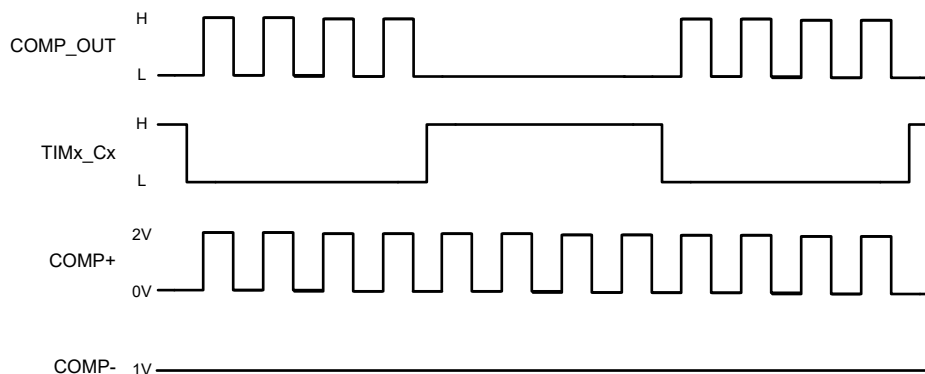
Figure 20-4. Blanking Mode Example Waveform
