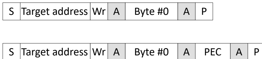
Figure 23-15. Send Byte Message with and without PEC
