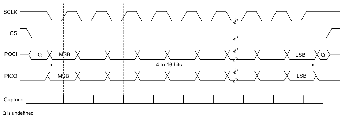
Figure 24-6. Motorola SPI Frame Format With SPO = 1 and SPH = 1
