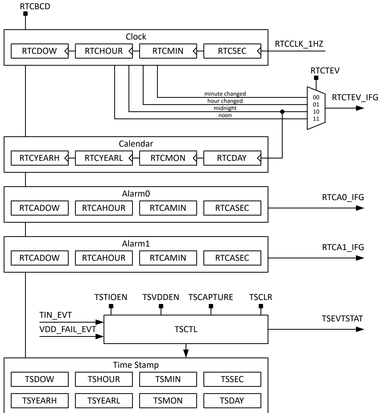
Figure 30-4. RTC Block Diagram and Timestamping
