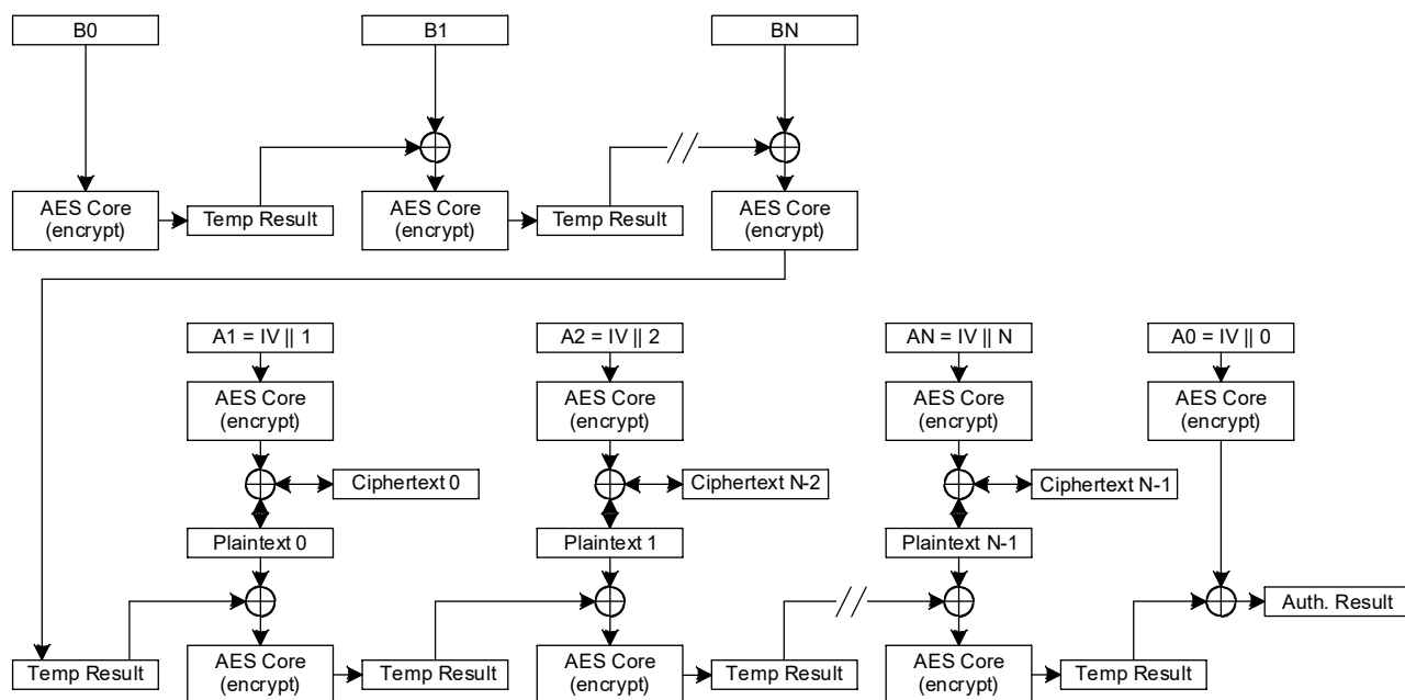
Figure 13-9. CCM Protocol Operation
