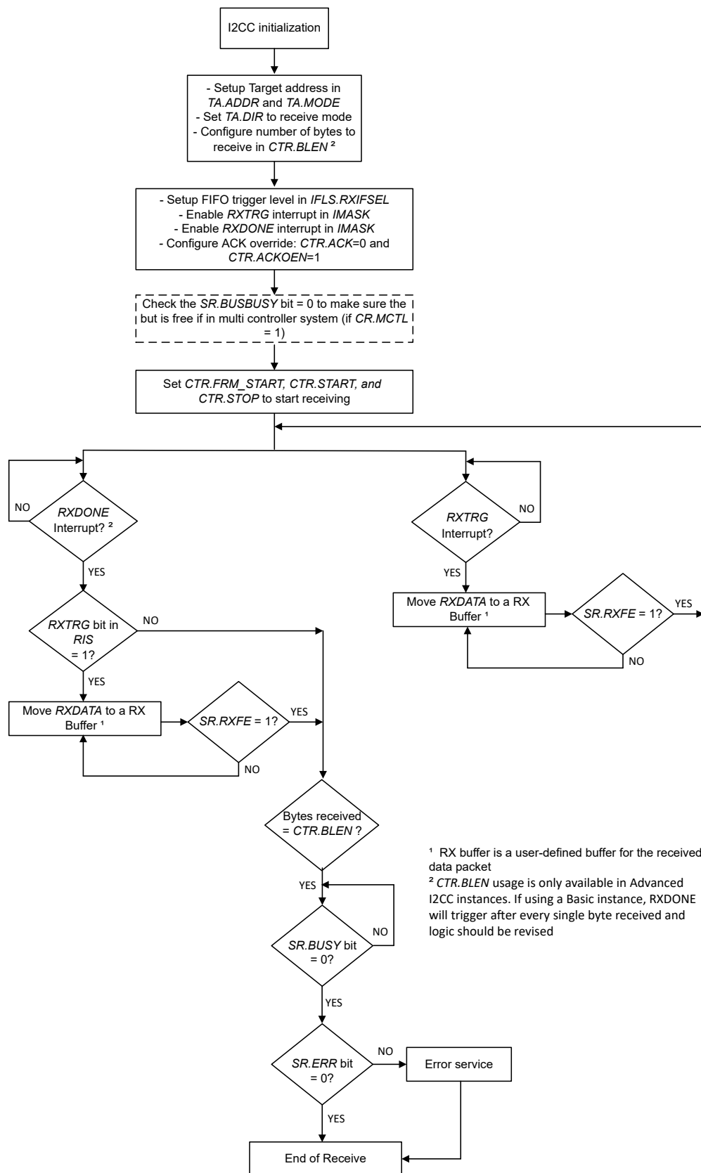
Figure 23-17. Controller Receive Mode
