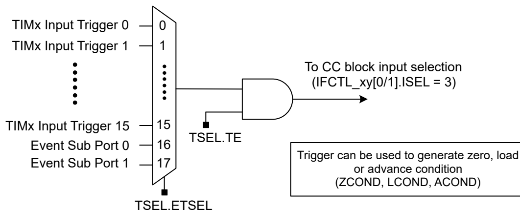
Figure 28-40. Secondary Timer Cross Trigger Input Configuration
