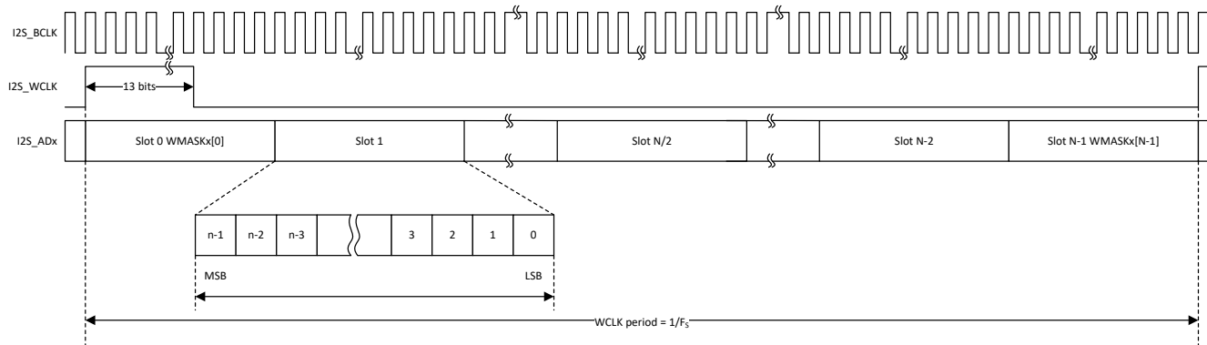
Figure 27-14. PCM Long Frame Format
