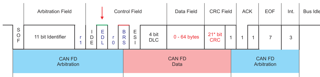
Figure 26-4. CAN FD Frame
