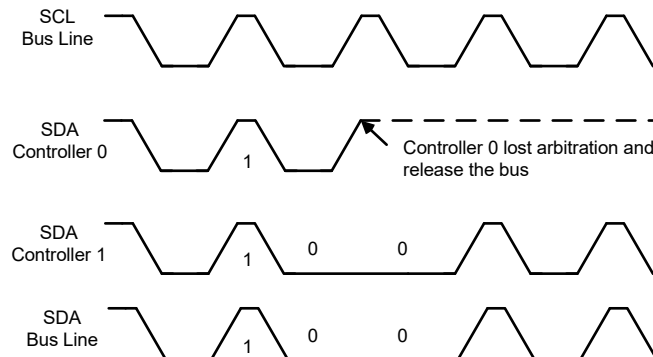
Figure 23-12. Arbitration Procedure Between Two Controller Transmitters
