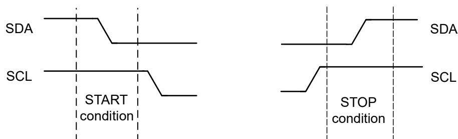
Figure 23-6. START and STOP Conditions
