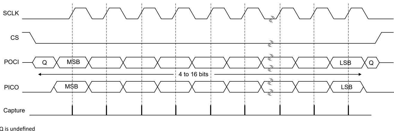
Figure 24-3. Motorola SPI Format With SPO = 0 and SPH = 0
