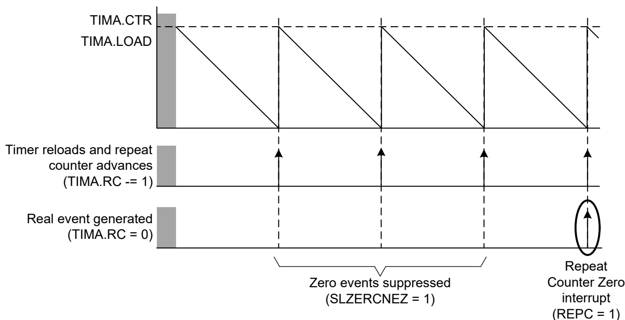
Figure 28-3. Event Suppressed by Repeat Counter with TIMx.RCLD = 4 in Down Counting Mode
