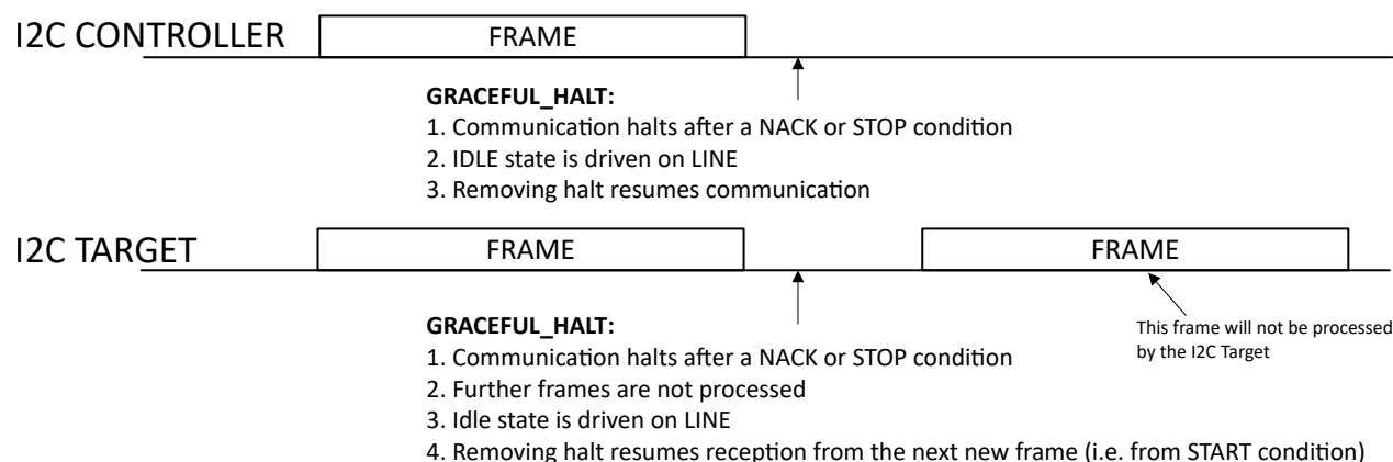
Figure 23-25. I2C Graceful Halt Emulation Behavior
