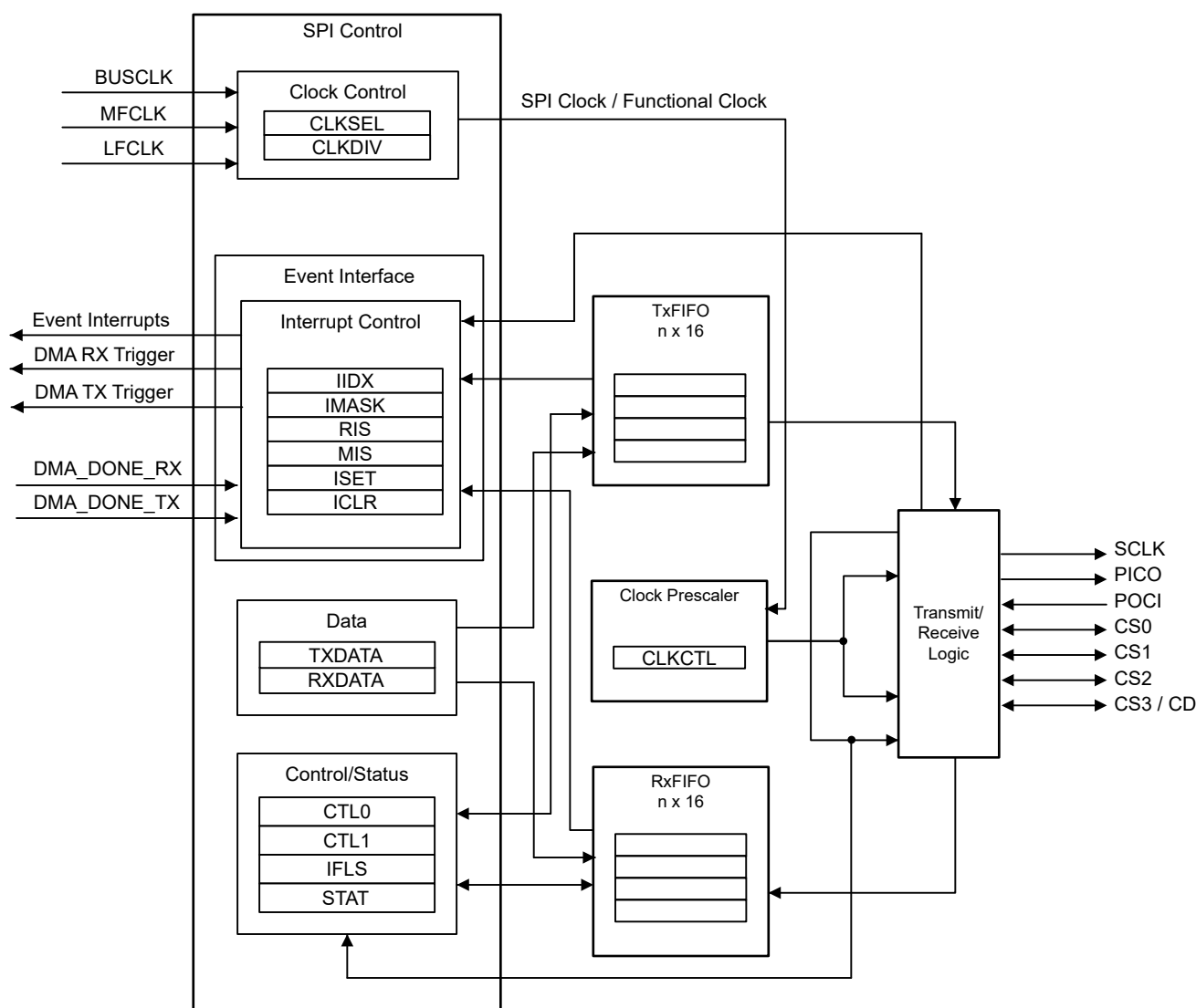
Figure 24-1. SPI Functional Block Diagram
