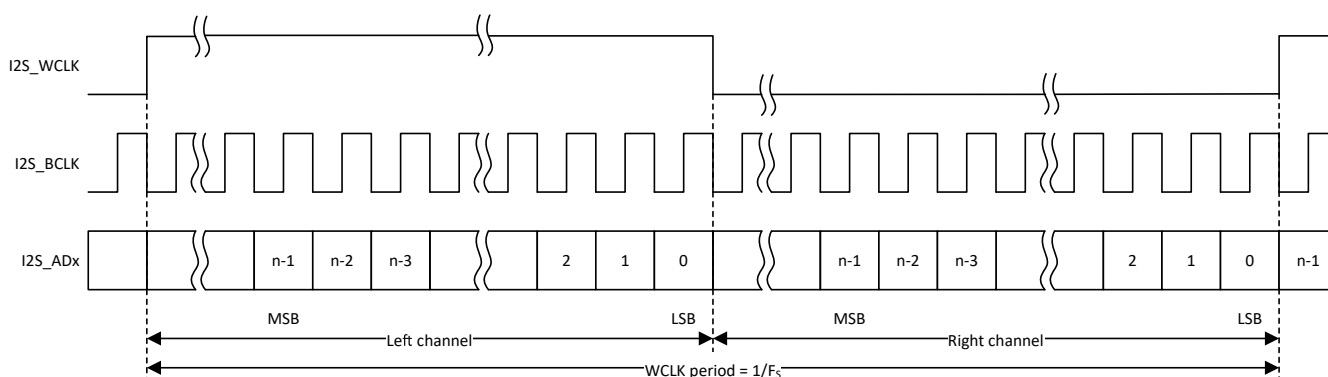
Figure 27-11. Right Justified Format
