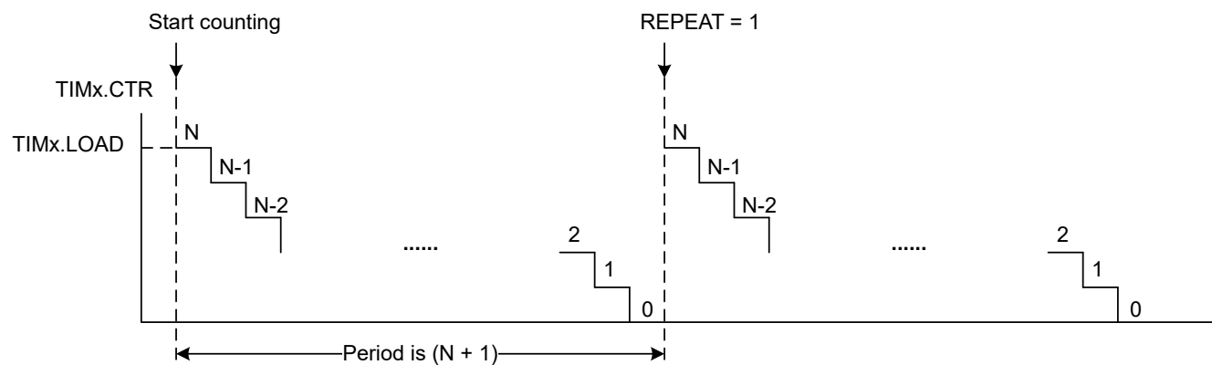
Figure 28-5. Down Counting Mode
