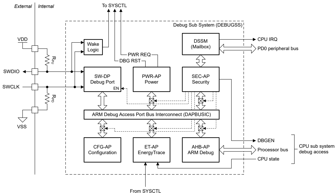
Figure 33-1. Debug Sub System Block Diagram
