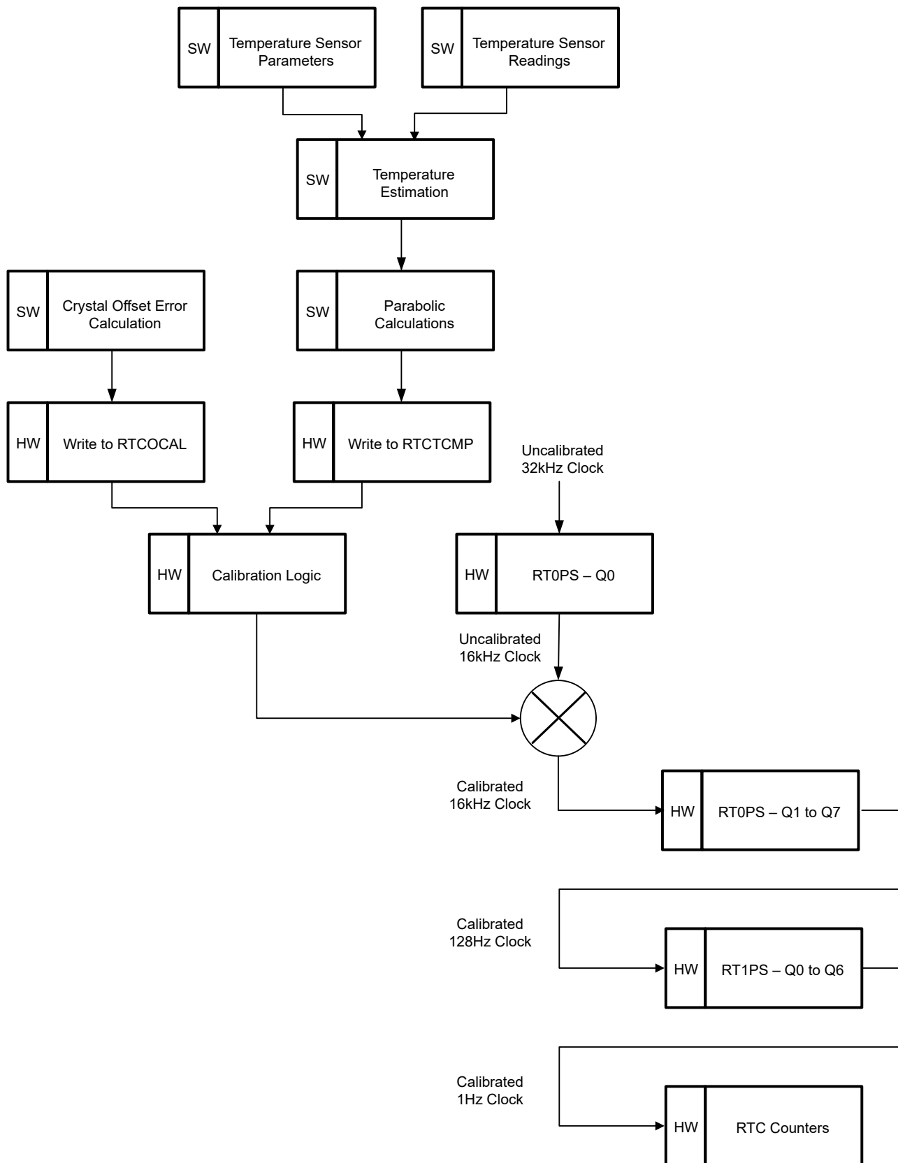
Figure 30-2. RTC Calibration
