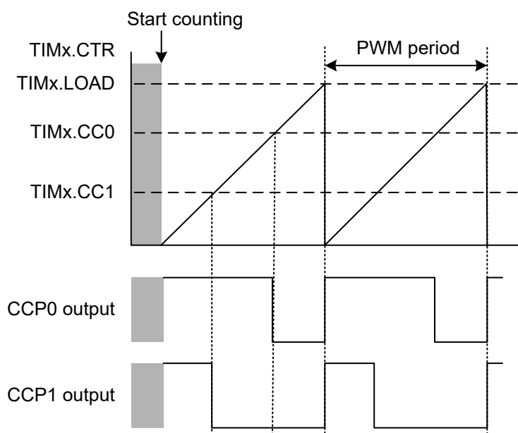
Figure 28-29. Edge-Aligned PWM Signals in Up-Counting Mode
