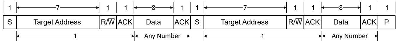
Figure 23-11. Data Format with Repeated Start
