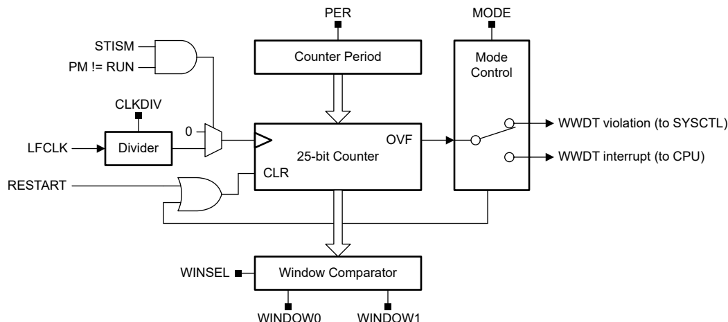
Figure 32-2. WWDT Diagram
