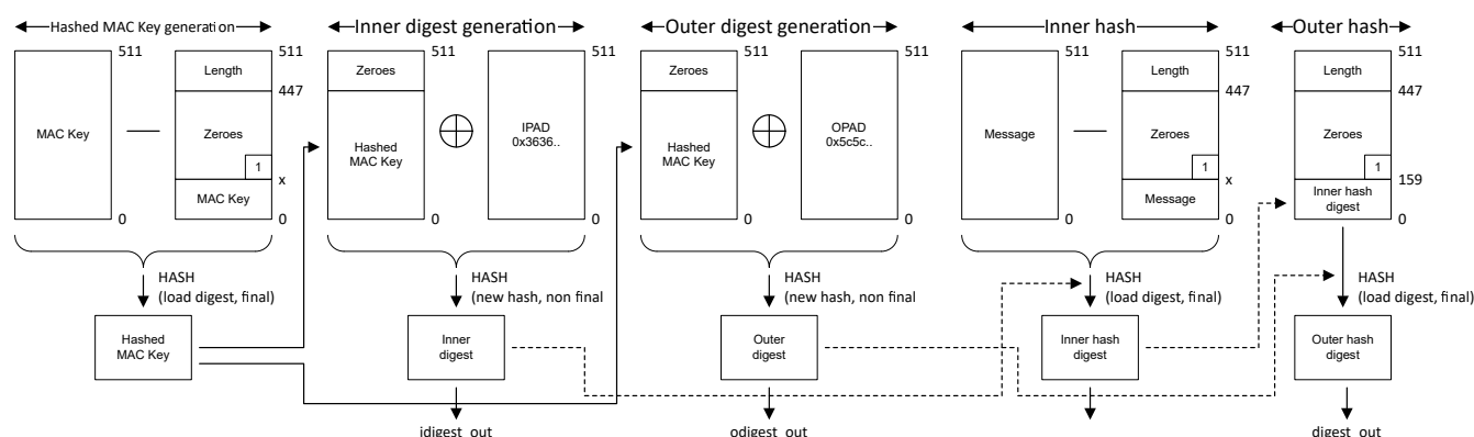
Figure 14-3. HMAC Processing with Long Key
