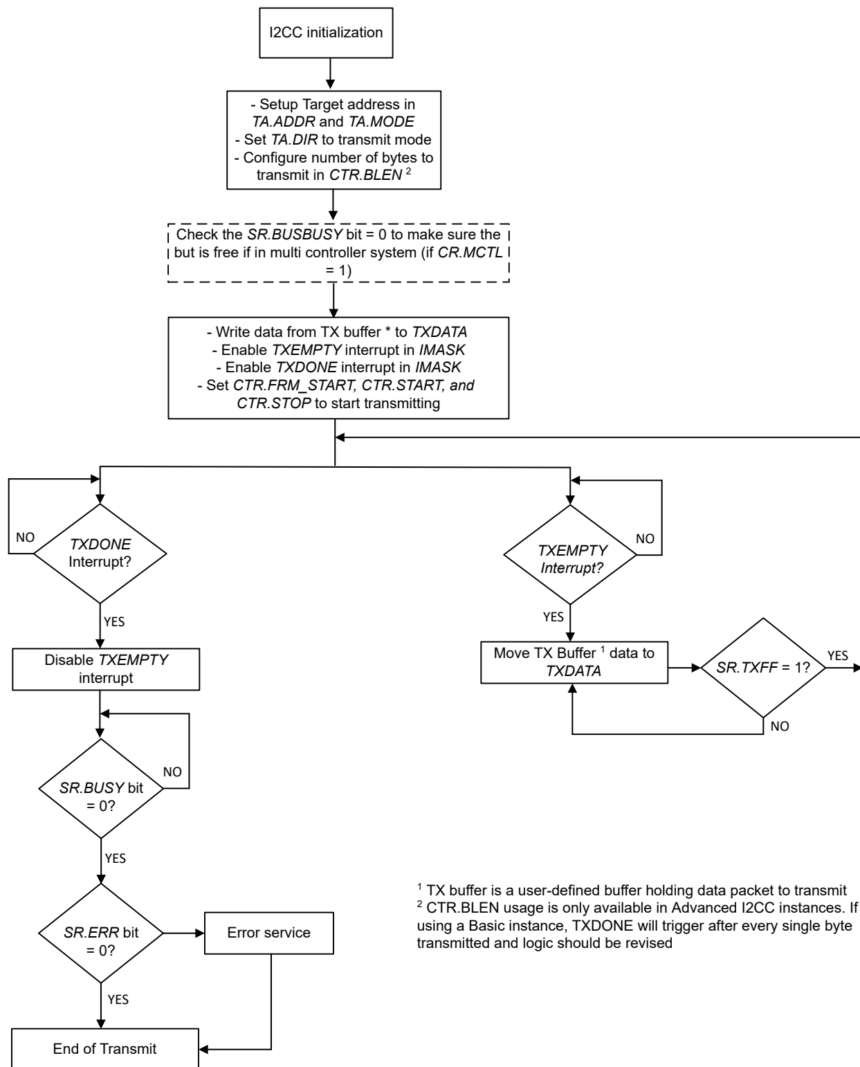
Figure 23-18. Controller Transmitter Mode using TXDONE
