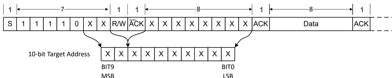
Figure 23-8. Data Format with 10-Bit Address
