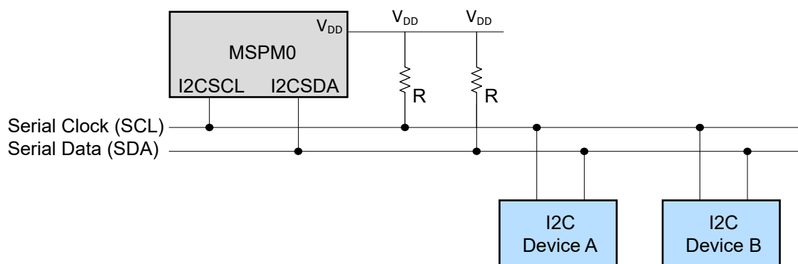
Figure 23-3. Bus Connection Diagram
