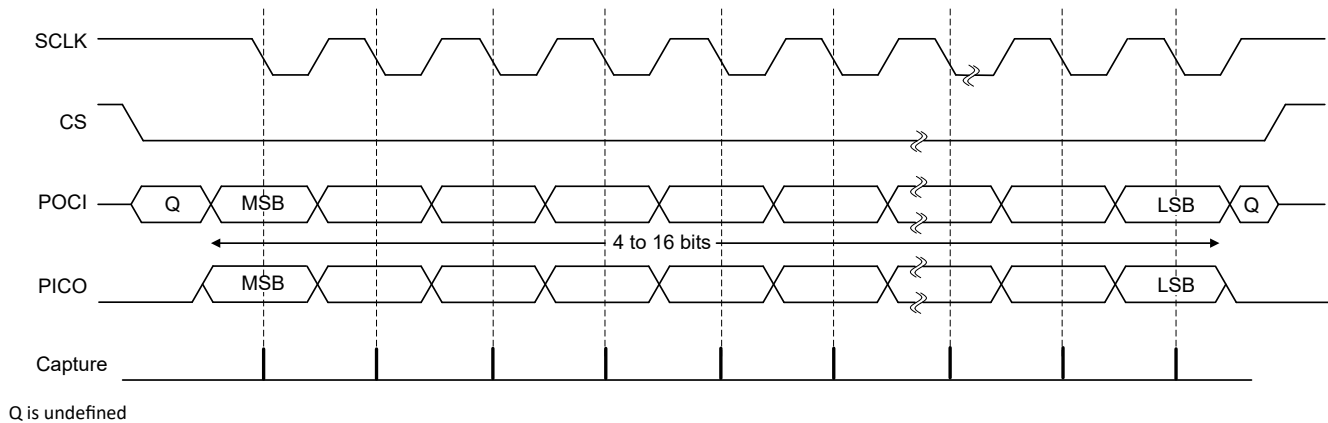
Figure 24-5. Motorola SPI Frame Format With SPO = 1 and SPH = 0
