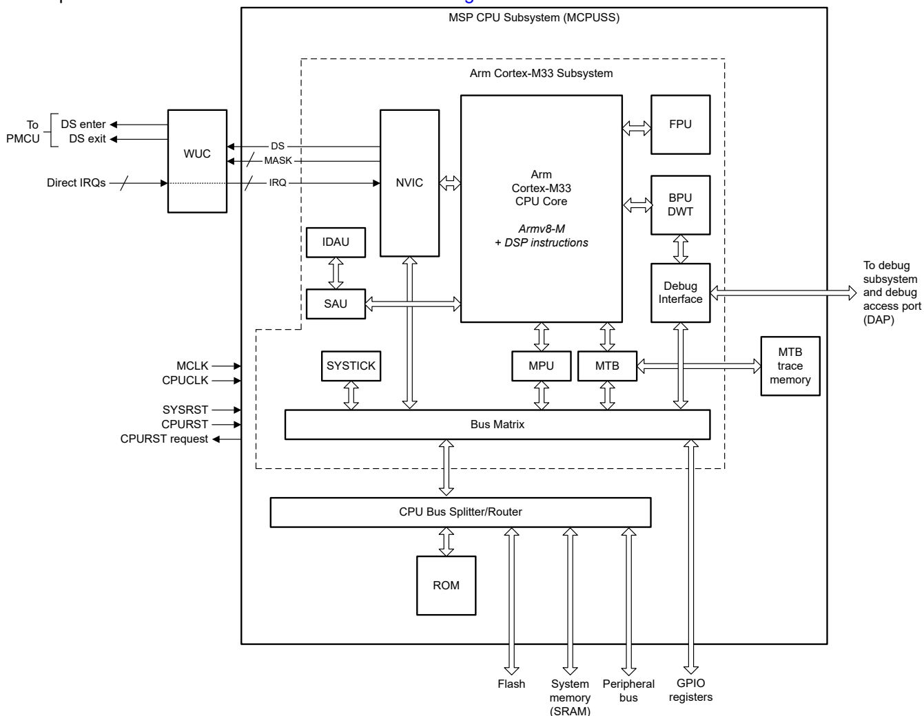
Figure 3-1. MSPM33Cxx MCPUSS Top Level Diagram
