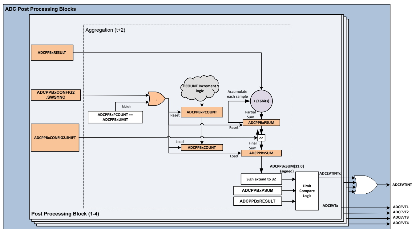
Figure 18-6. ADC Post-Processing Blocks (PPB) Block Diagram
