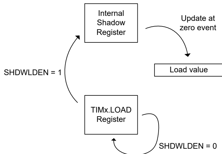
Figure 28-24. Load value updates for TIMx instances when EN=1
