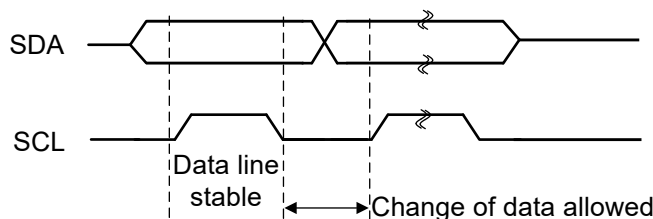
Figure 23-5. Data Change Period
