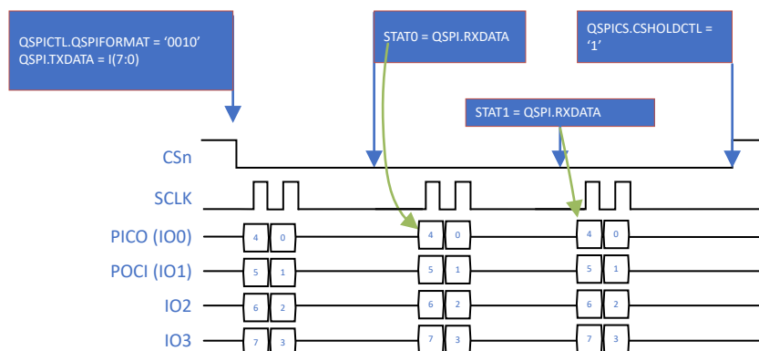
Figure 25-7. Status Frame Access-QPI Mode
