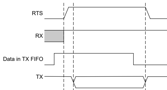
Figure 22-11. RS485 Data Exchange
