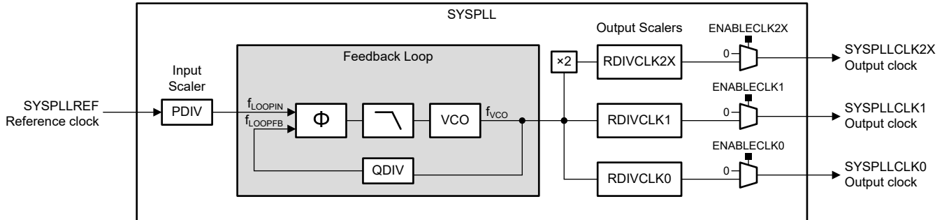
Figure 2-6. SYSPLL Diagram
