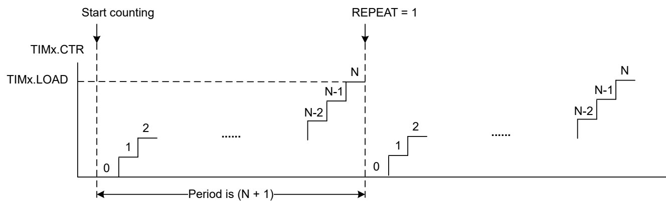
Figure 28-9. Up Counting Mode
