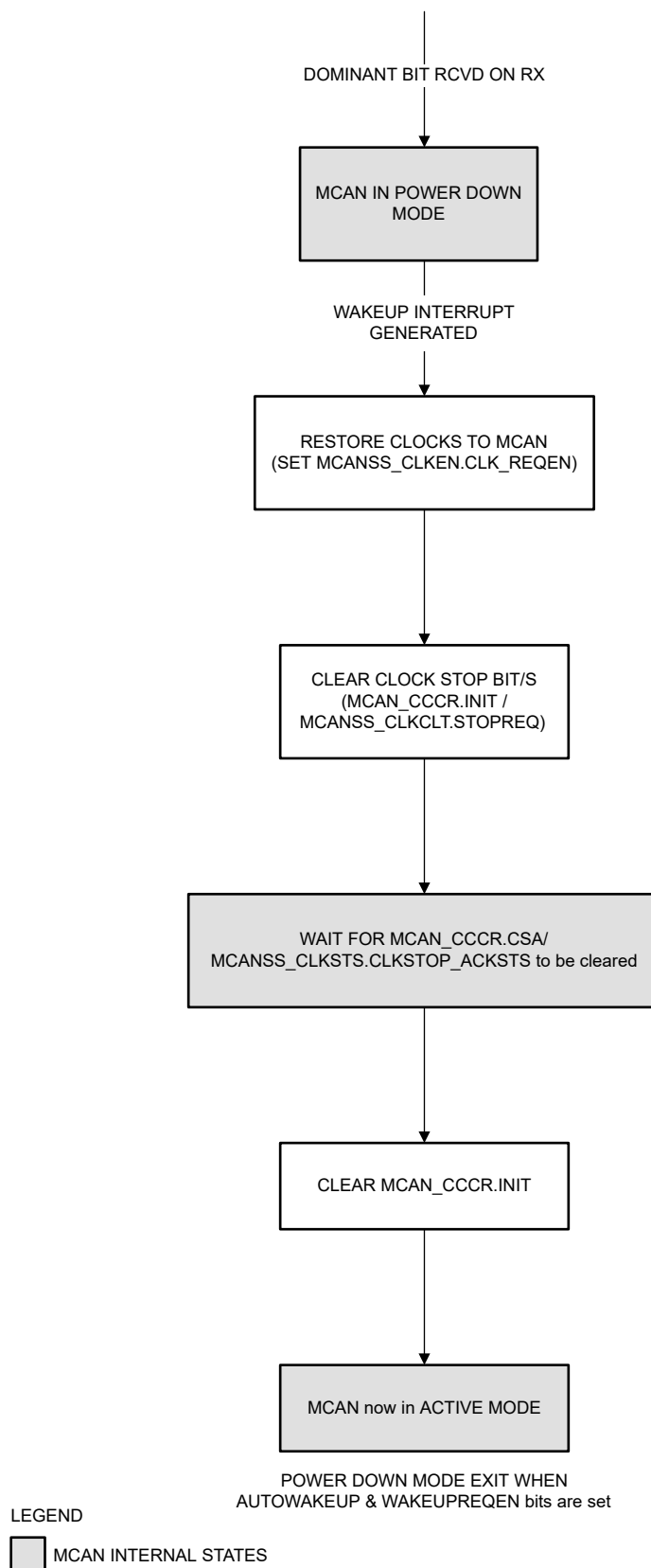
Figure 26-10. Auto Wakeup Enabled Exit from Power Down
