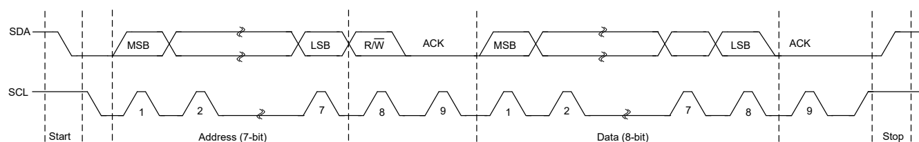
Figure 23-4. Module Data Transfer
