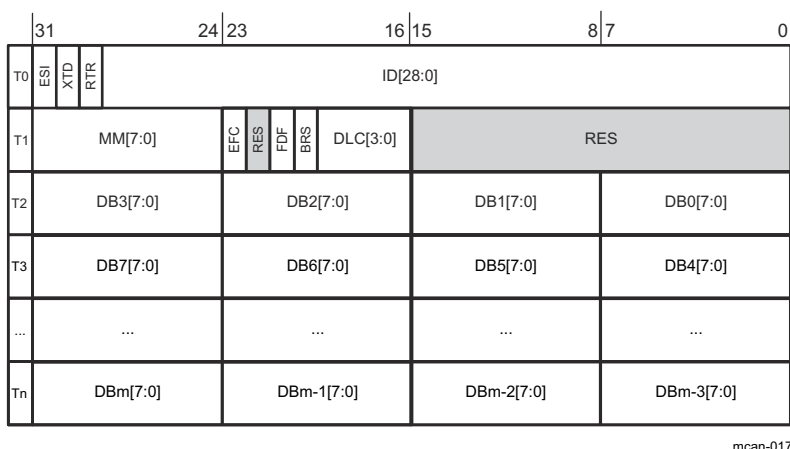
Figure 26-22. Tx Buffer Element Structure
