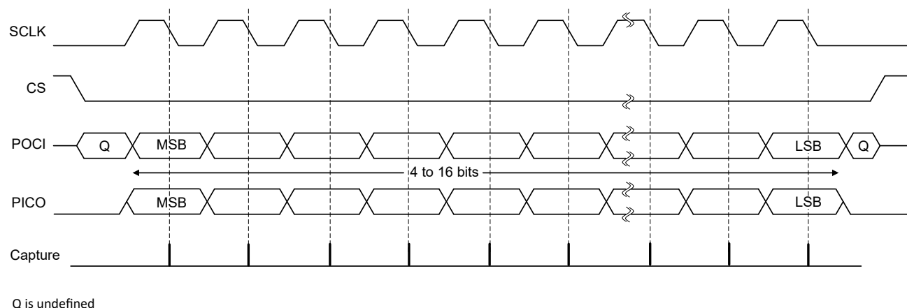
Figure 24-4. Motorola SPI Frame Format With SPO = 0 and SPH = 1
