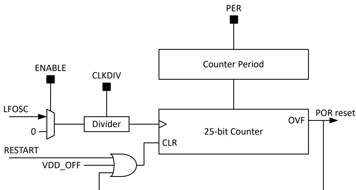
Figure 31-1. Independent Watchdog Timer (IWDT) Block Diagram
