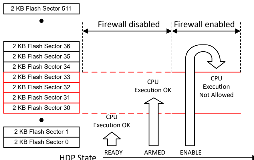
Figure 11-6. HDP execution mechanism
