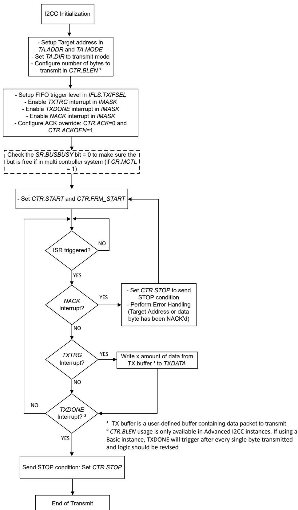
Figure 23-19. Controller Transmitter Mode using TXTRG
