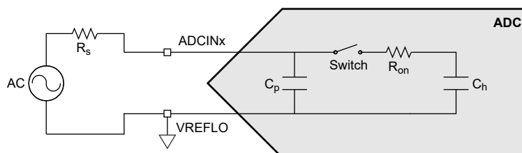
Figure 18-4. Single-Ended Input Model
