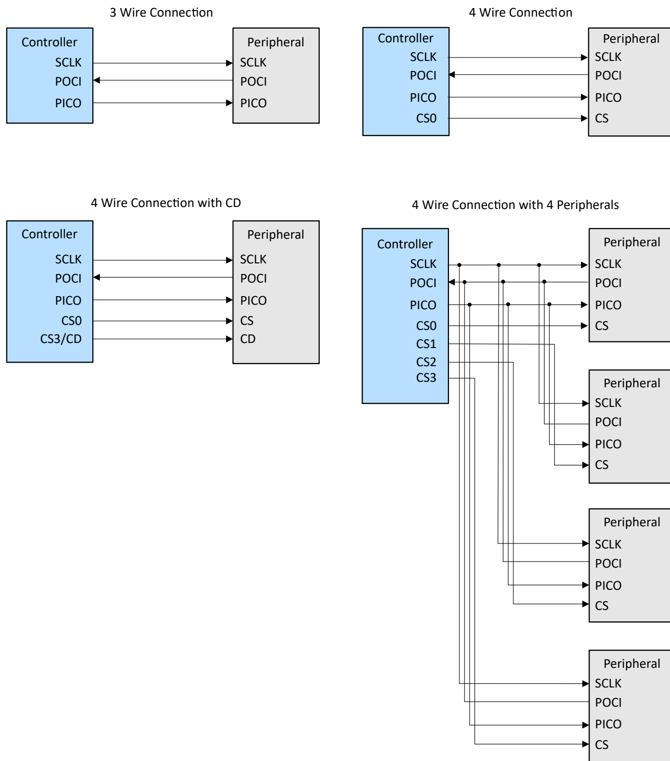
Figure 24-2. External Connections for Different SPI Configurations
