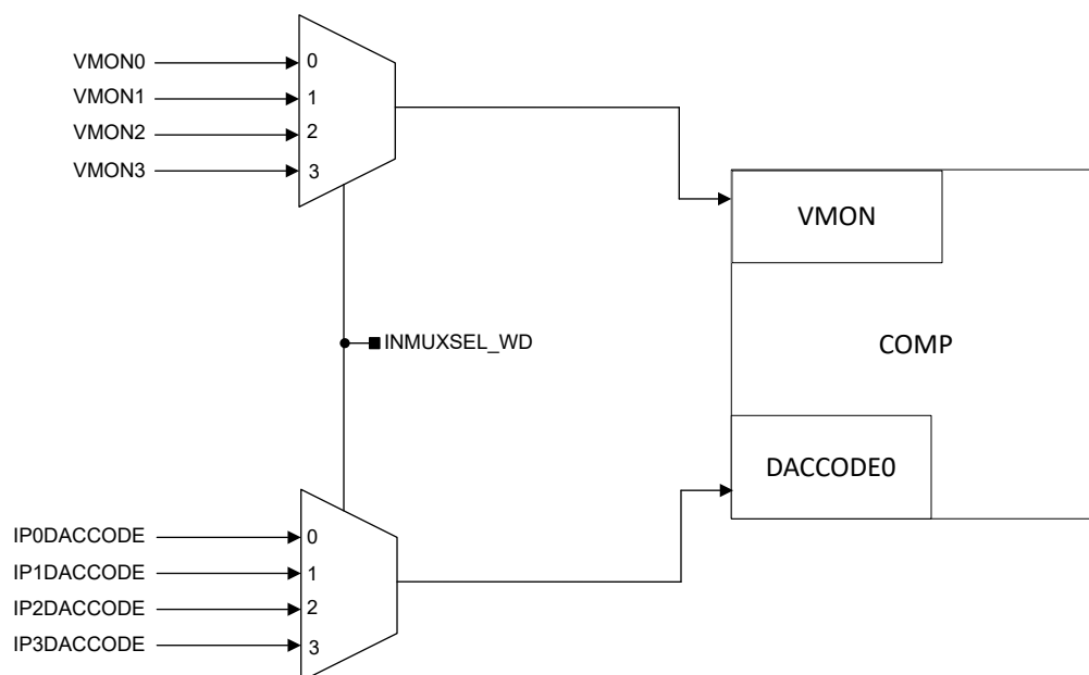
Figure 20-7. Analog signal comparison diagram
