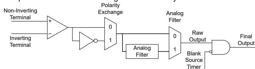
Figure 20-3. Blanking Mode Block Diagram
