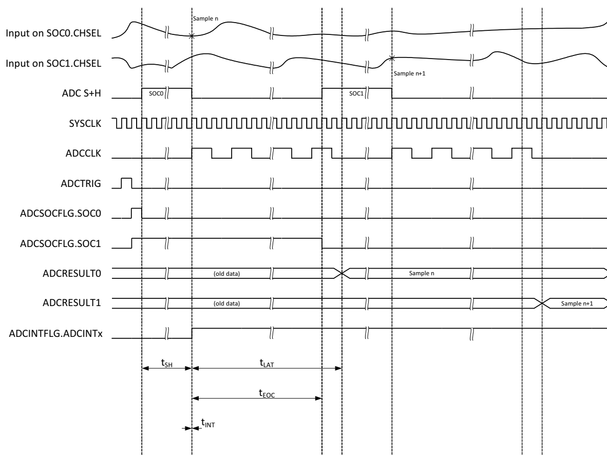
Figure 18-7. ADC Timings for 12-bit Mode in Early Interrupt Mode
