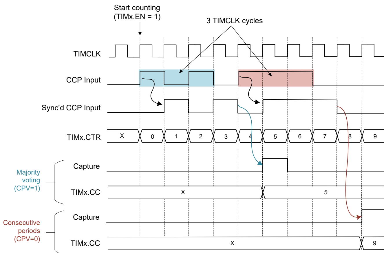
Figure 28-13. Consecutive Period and Majority Voting for Input Glitch Filtering using FP = 0 (3 TIMCLK cycles)
