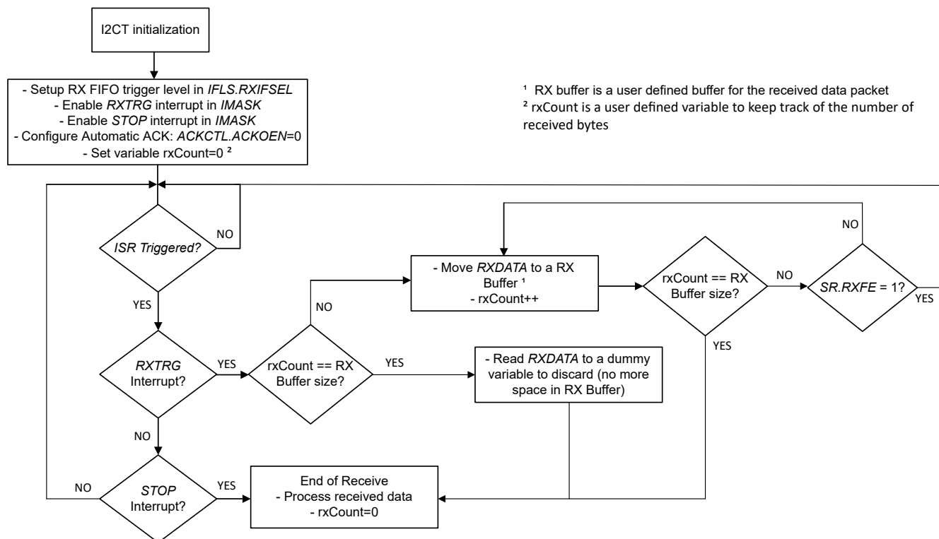
Figure 23-21. Target Receiver Mode using RXTRG and Automatic ACK
