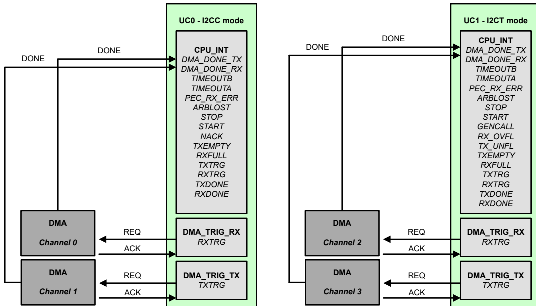
Figure 23-24. I²C DMA Trigger and Status Example
