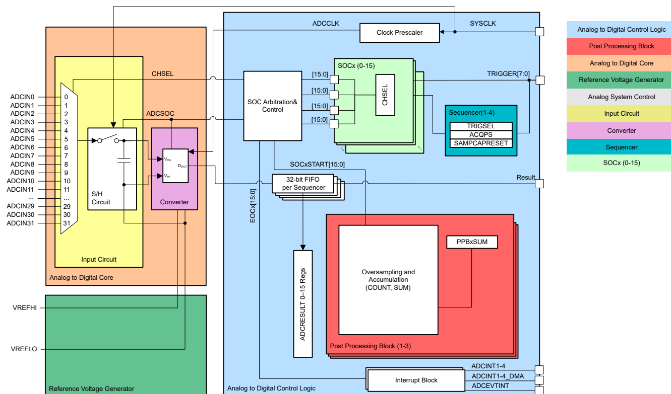
Figure 18-1. ADC Module Block Diagram
