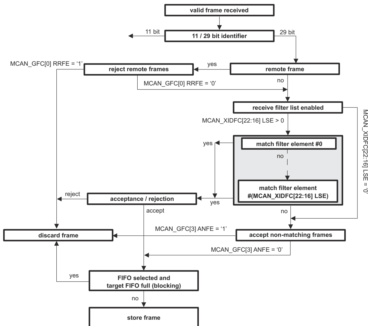
Figure 26-17. Extended Message ID Filter Path
