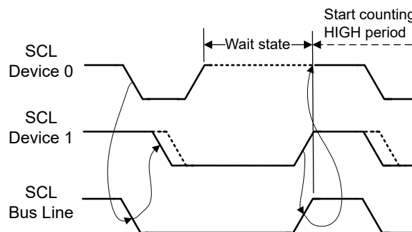
Figure 23-13. Clock Synchronization
