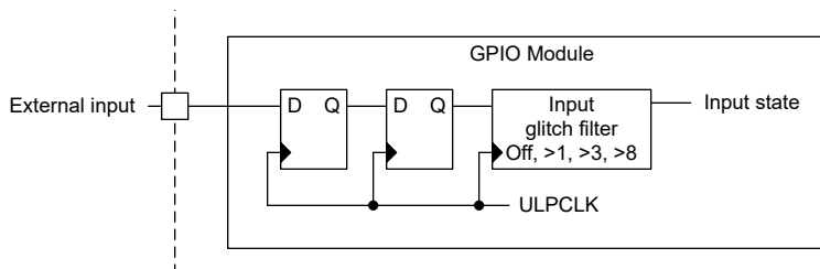
Figure 10-2. GPIO Input Synchronizer
