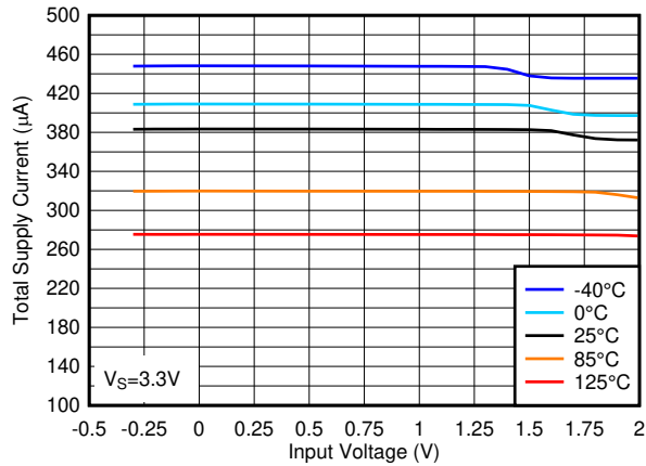
Figure 2-3. Total Supply Current vs. Input Voltage at 3.3V
