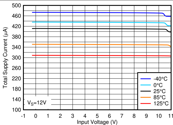
Figure 2-5. Total Supply Current vs. Input Voltage at 12V
