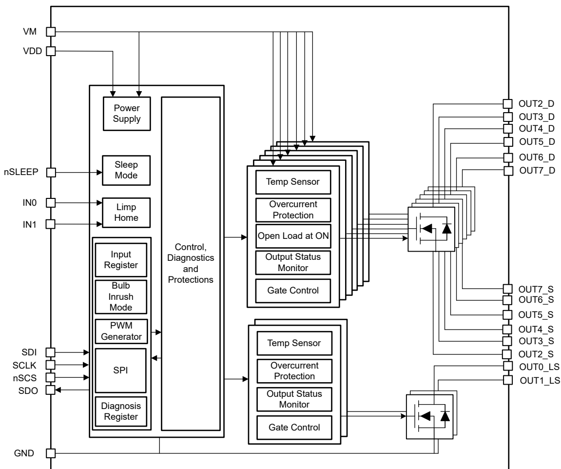
Figure 7-1. DRV81602-Q1 Functional Block Diagram
