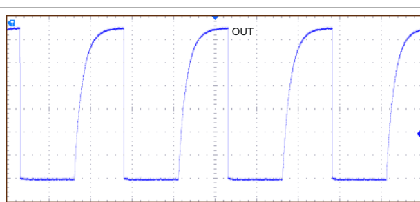
Figure 7-3. 10-kHz Switching Magnetic Field
