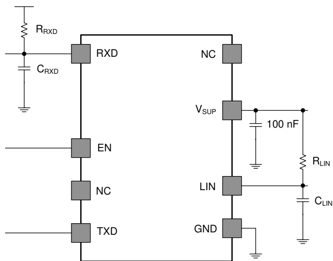
Figure 6-17. Wake-up through LIN
