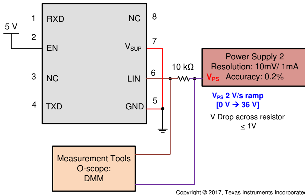
Figure 6-10. Test Circuit for I_{BUS\_NO\_BAT} Loss of Battery
