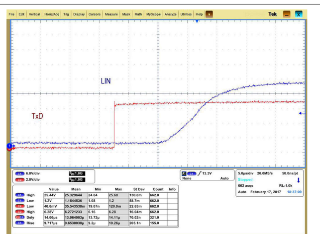
Figure 8-3. Dominant to Recessive Propagation
