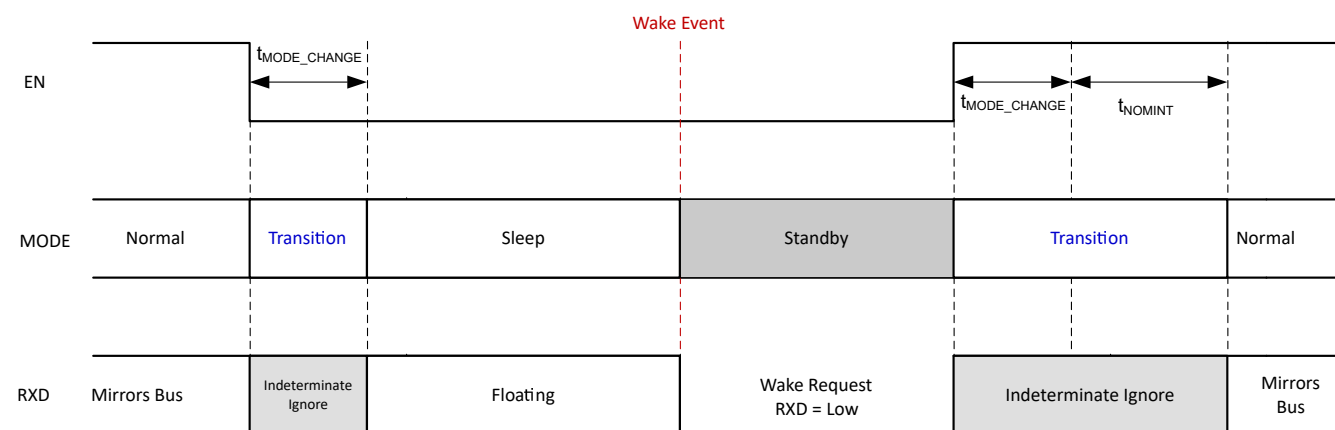
Figure 6-15. Mode Transitions
