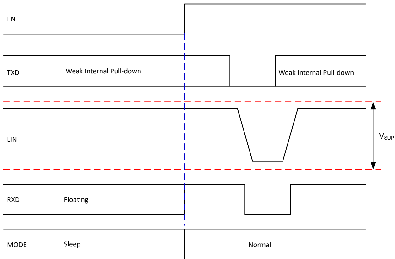
Figure 6-16. Wake-up Through EN
