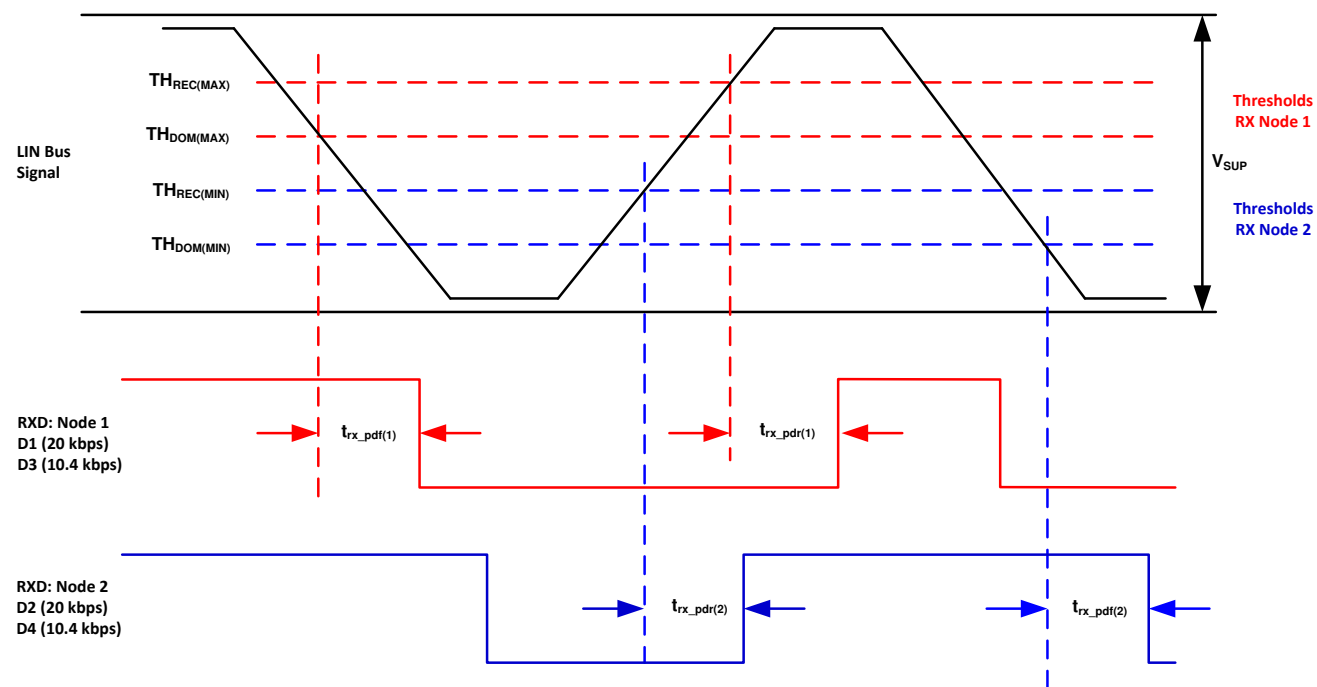
Figure 6-14. Propagation Delay
