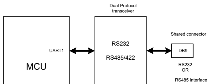
THVD4431 Simplified Schematic
