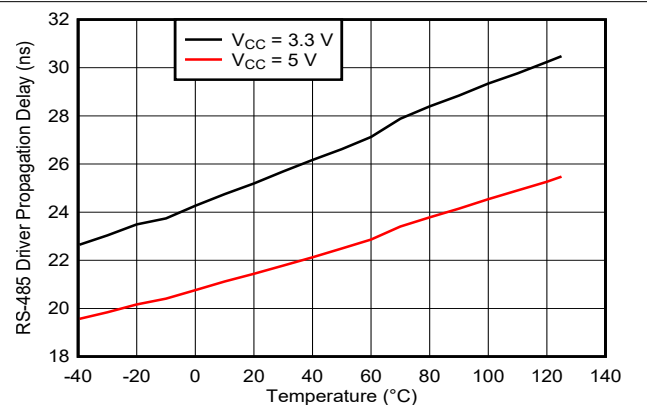
Figure 5-12. RS-485 20Mbps Driver Propagation Delay vs Temperature
