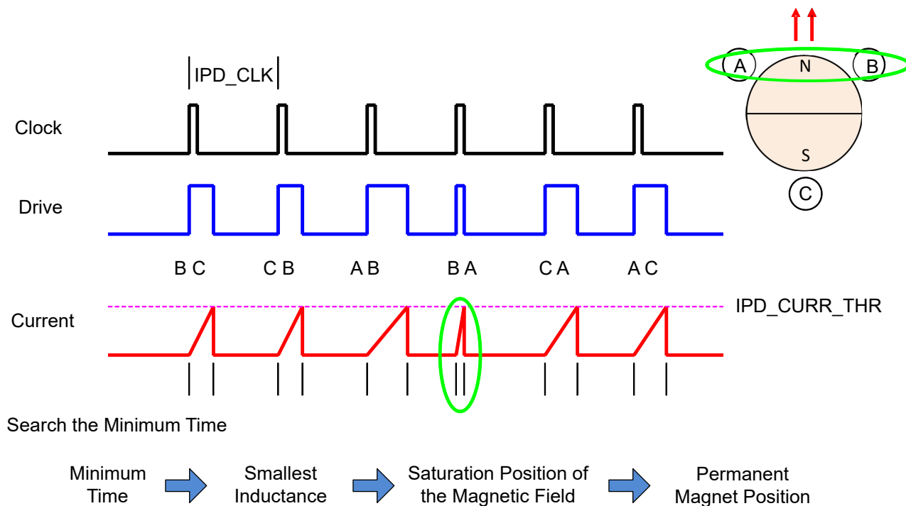
Figure 6-33. IPD Function
