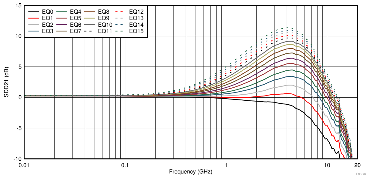
Figure 5-14. Downstream-to-Upstream EQ Settings Curves
