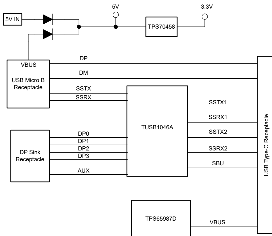
Figure 1-1. Block Diagram
