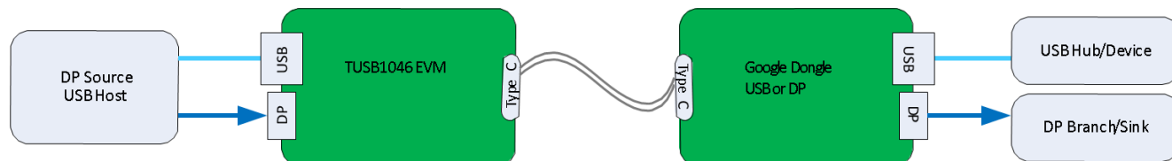
Figure 2-1. Test Board Setup
