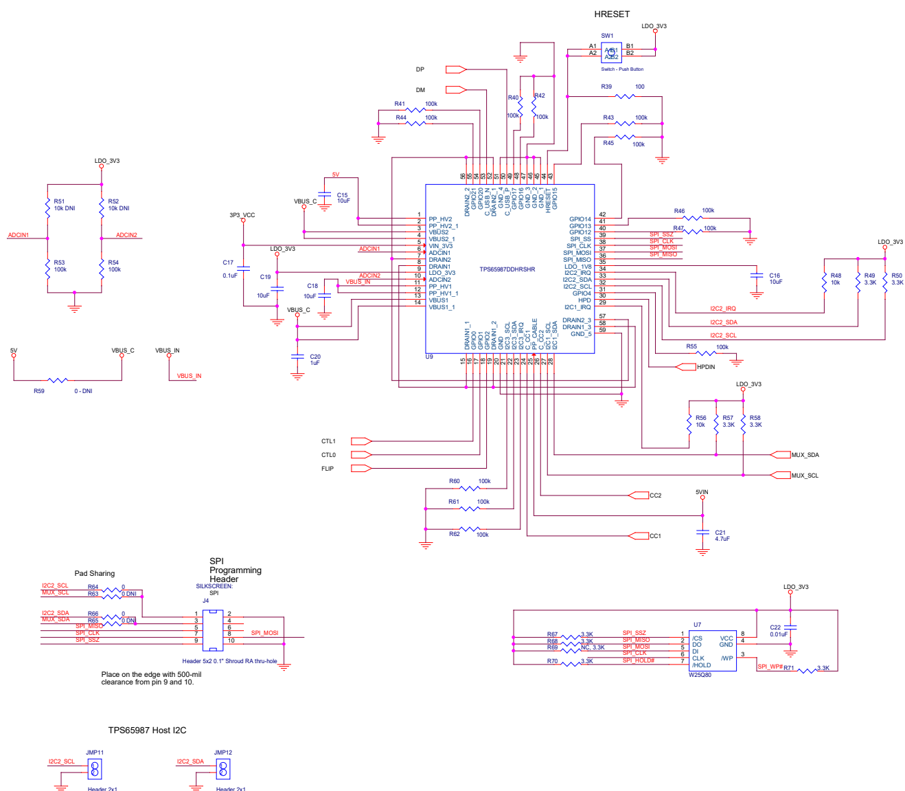
Figure 4-4. TUSB1046EVM Schematics (3 of 4)
