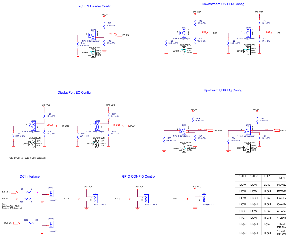
Figure 4-3. TUSB1046EVM Schematics (2 of 4)
