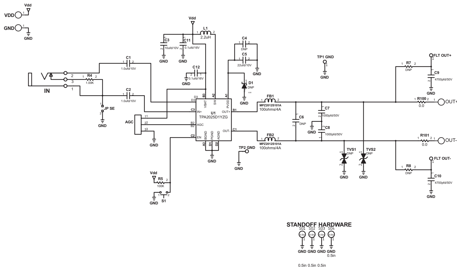
Figure 1. TPA2025D1EVM Schematic
