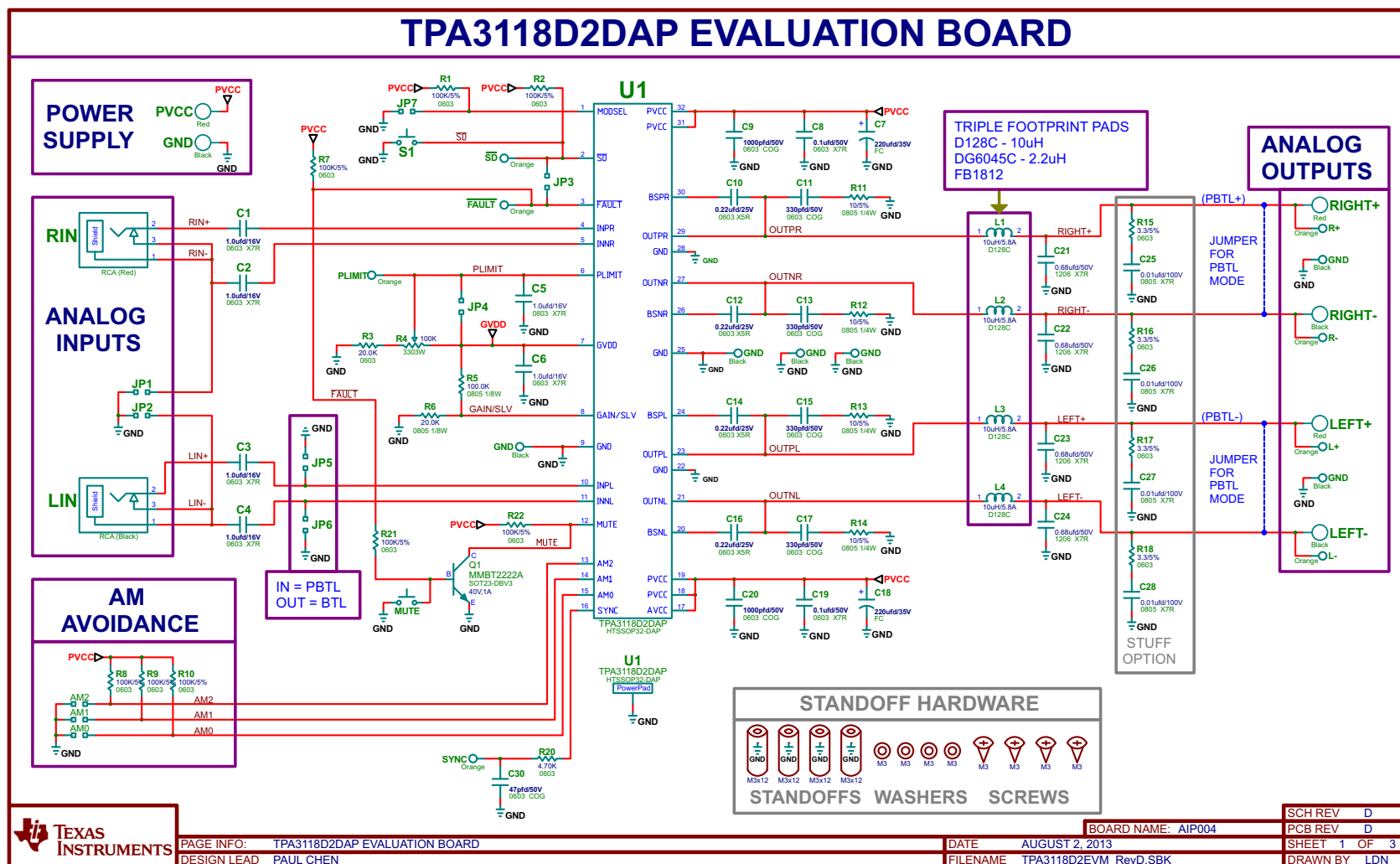
Figure 3. TPA3118D2EVM Schematic
