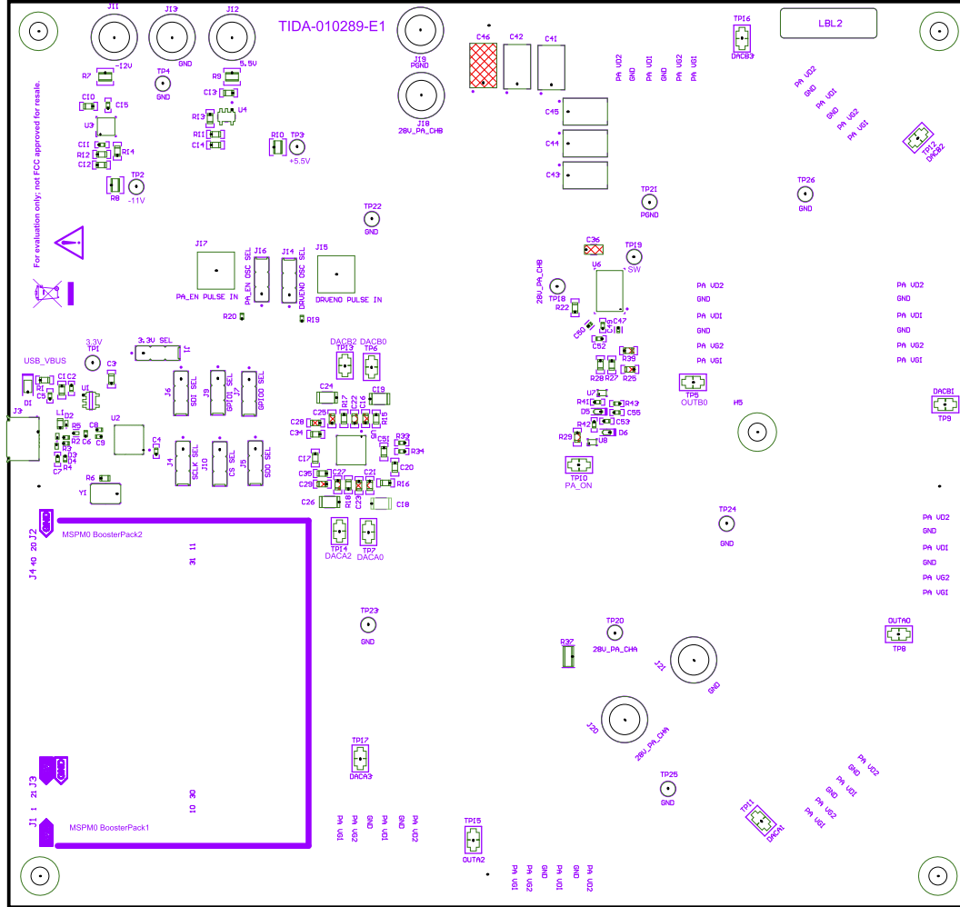
View from Top side (Scale 1:1.18)
