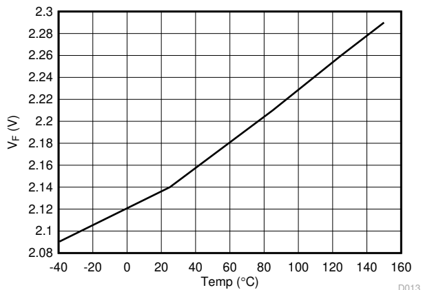
Figure 6-15. Forward voltage drop versus Temperature
