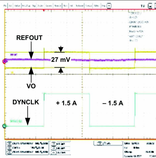
Figure 25. Transient Waveform
