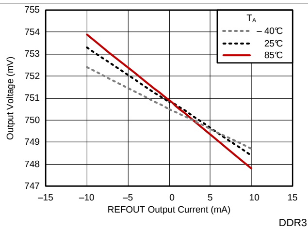
Figure 11. REFOUT Load Regulation
