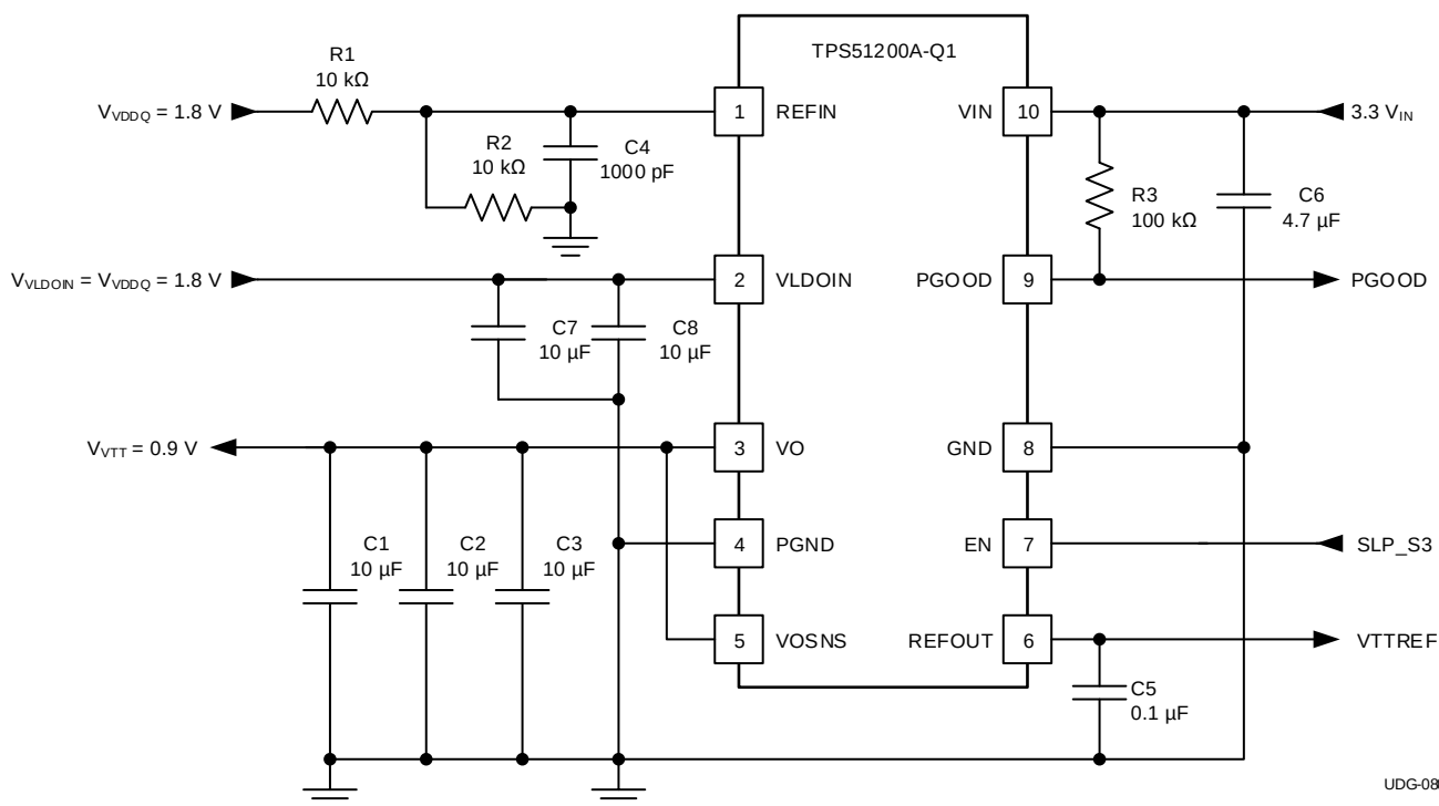
Figure 26. 3.3- V_{IN} , DDR2 Configuration
