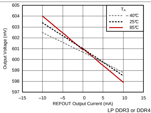
Figure 13. REFOUT Load Regulation
