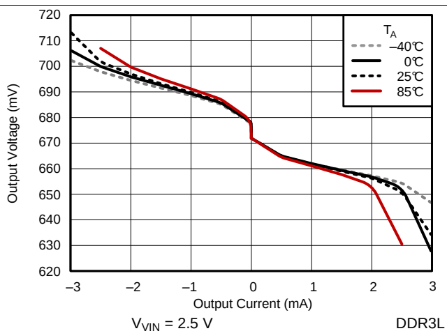
Figure 9. Load Regulation
