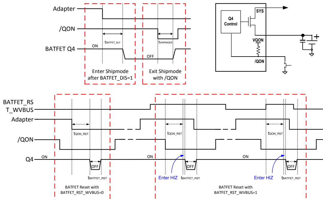
Figure 9-7. \overline{\text{QON}} Timing
