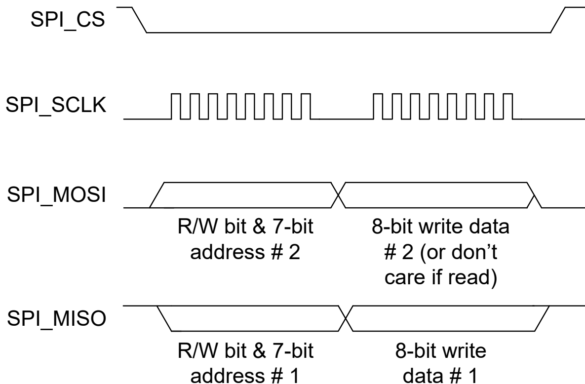
Figure 14-9. SPI Transaction #2 Without CRC
