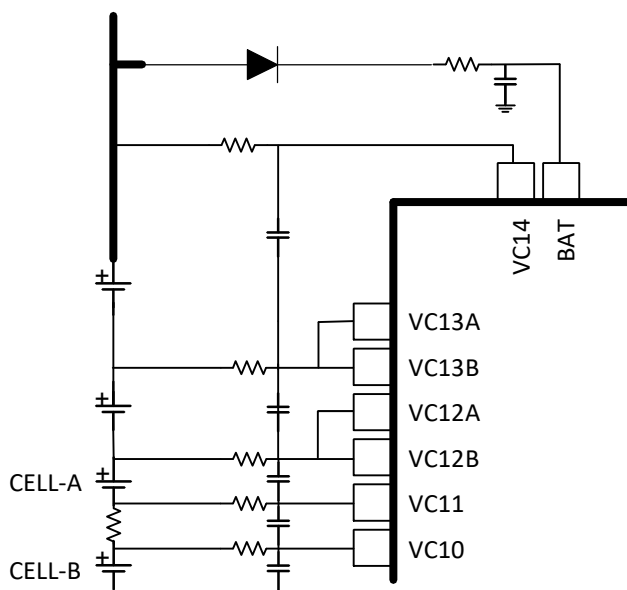
Figure 10-1. Using Cell Input Pins for Interconnect Measurement
