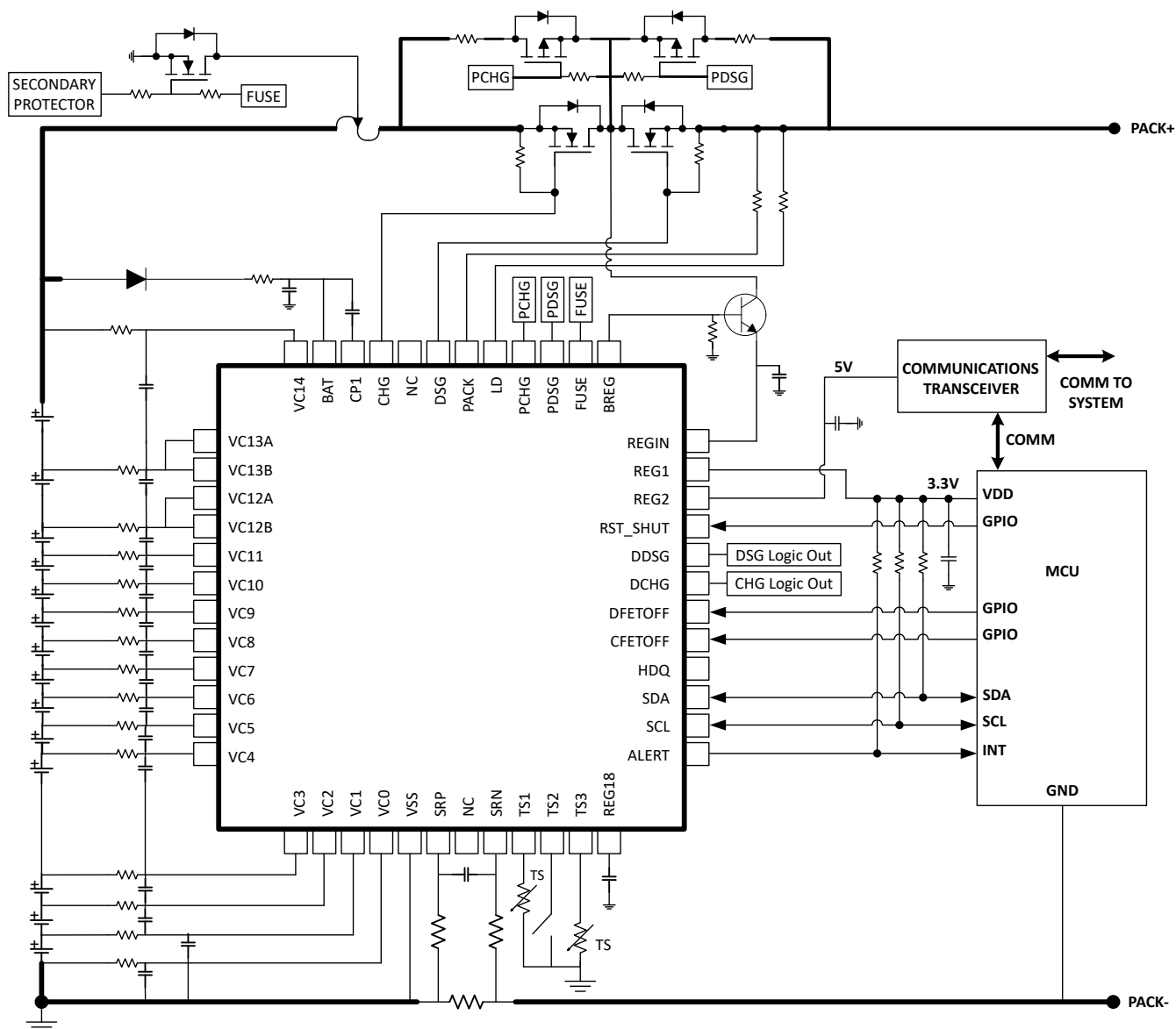
Figure 16-1. BQ769142 14-Series Cell Typical Implementation (Simplified Schematic)
