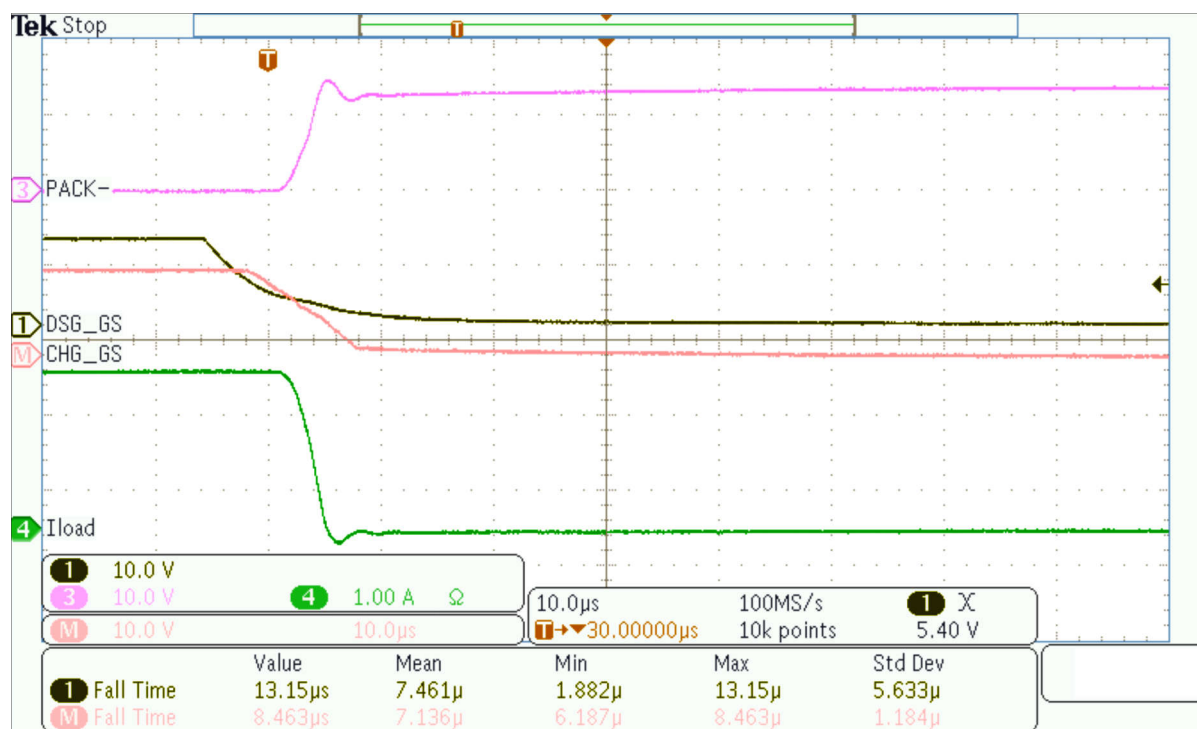
Figure 8-6. Moderate Speed DSG FET Turn-Off, Using a 1.35-k \Omega Series Gate Resistor, and a 2A Load between PACK+ and PACK–.
