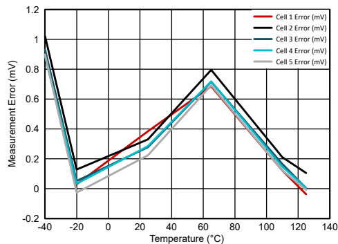
Figure 6-6. Cell Voltage Measurement Error vs. Temperature with Cell Voltage = 2.0 V
