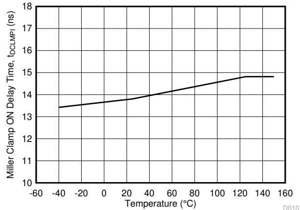
Figure 5-22. t_{DCLMPI} Miller Clamp ON Delay Time vs Temperature
