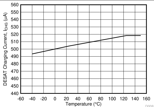
Figure 5-28. I_{\text{CHG}} DESAT Charging Current vs Temperature
