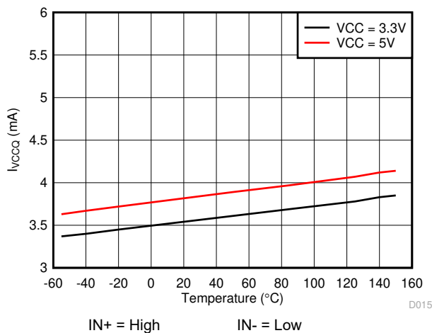
Figure 5-5. I_{VCCQ} Supply Current vs Temperature
