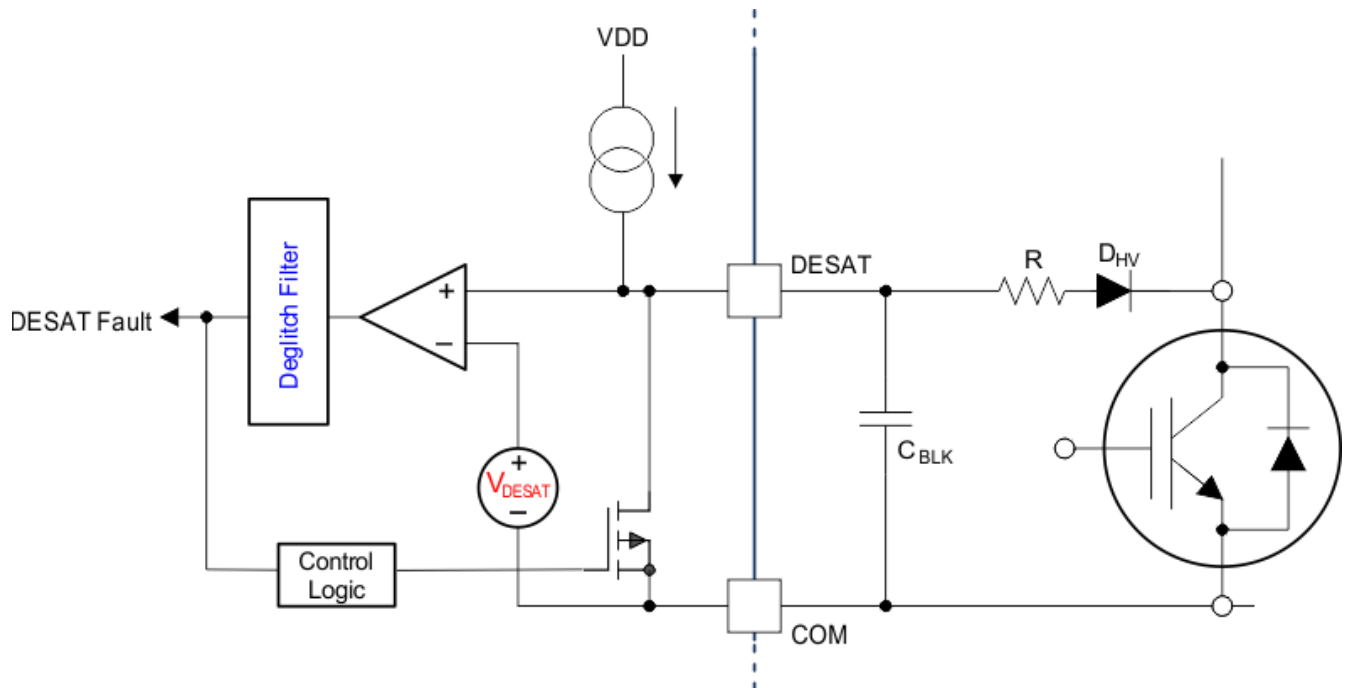
Figure 7-5. DESAT Protection
