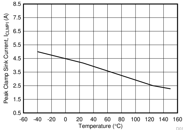
Figure 5-21. I_{CLMPI} Miller Clamp Sink Current vs Temperature
