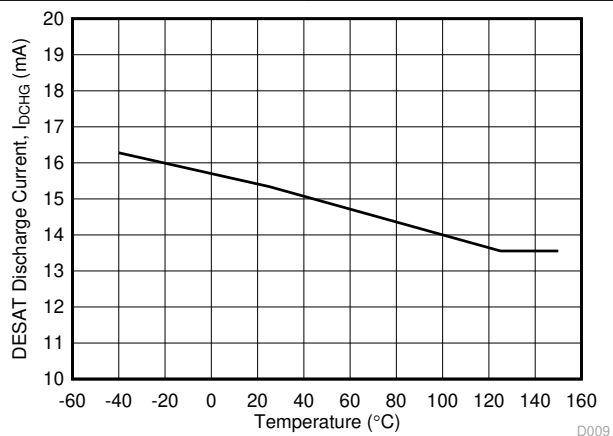
Figure 5-29. I_{\text{DCHG}} DESAT Discharge Current vs Temperature
