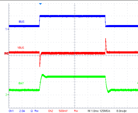
Figure 9-6. OTG Startup at 500-mA Load
