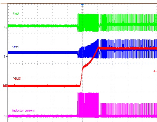
Figure 9-3. Buck Mode PFM with OOA
