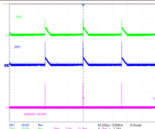
Figure 9-4. Buck Mode PFM without OOA
