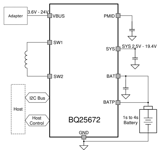
Simplified Schematic
