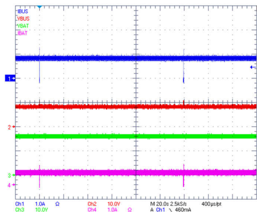
Figure 9-9. MPPT Operation
