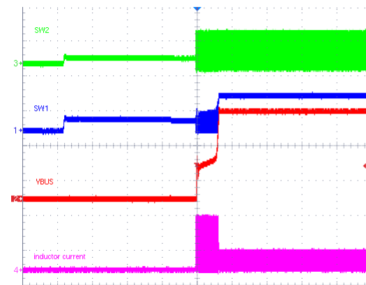
Figure 9-4. Buck Mode PFM without OOA
