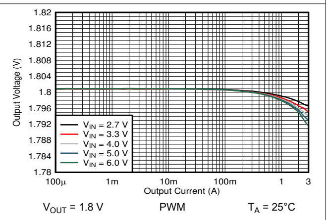
Figure 9-13. Output Voltage Versus Output Current
