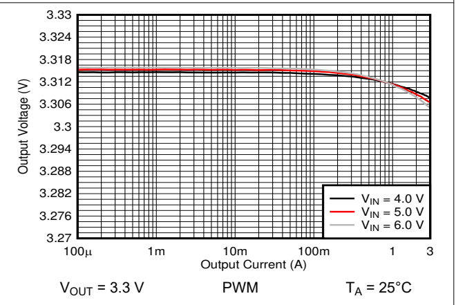
Figure 9-11. Output Voltage Versus Output Current
