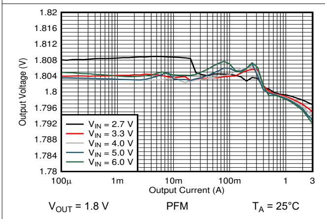
Figure 9-12. Output Voltage Versus Output Current
