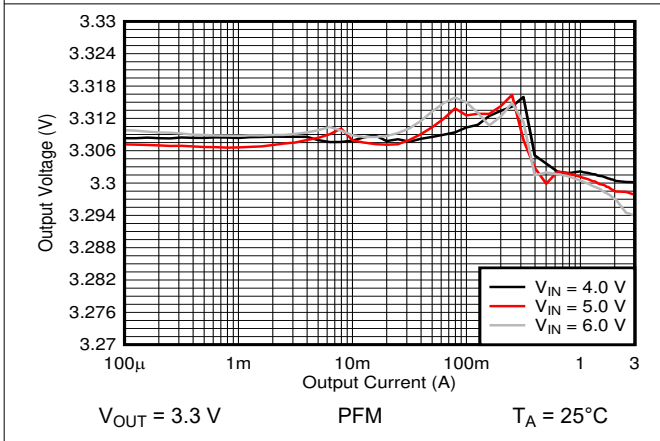
Figure 9-10. Output Voltage Versus Output Current
