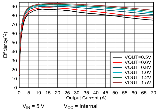
Figure 5-1. TPSM8D6C24 Efficiency vs Output Current
