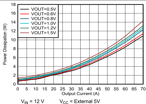
Figure 5-8. TPSM8D6C24 Power Dissipation vs Output Current
