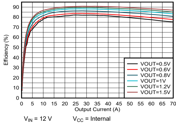
Figure 5-3. TPSM8D6C24 Efficiency vs Output Current
