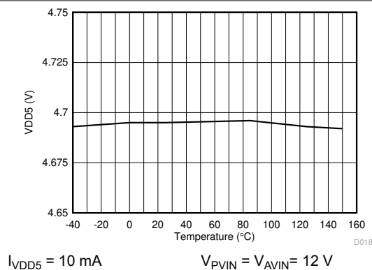
Figure 5-12. VDD5 Voltage vs Junction Temperature
