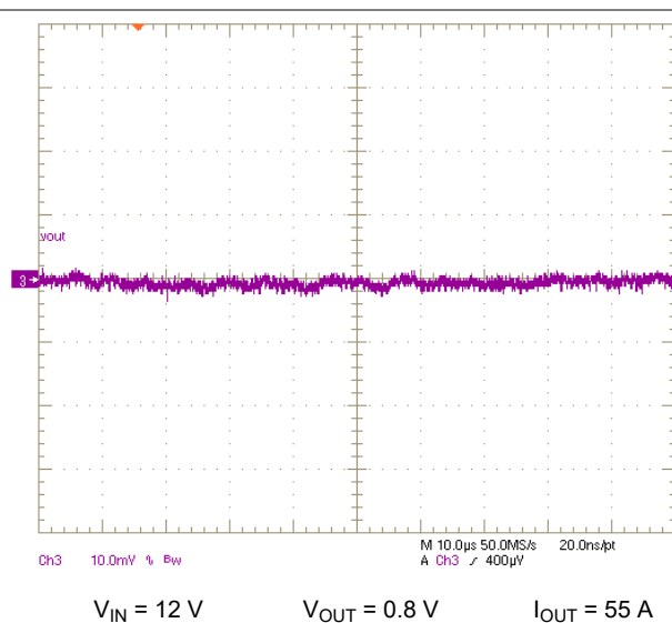
Figure 8-17. V_{OUT} Steady-State Ripple
