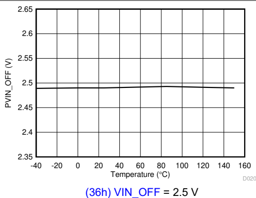
Figure 5-15. Turn-Off Voltage vs Junction Temperature
