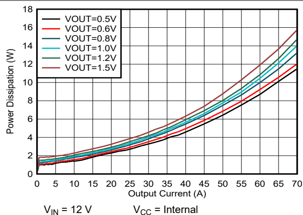
Figure 5-7. TPSM8D6C24 Power Dissipation vs Output Current
