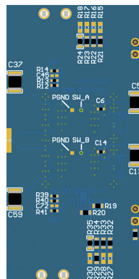
Figure 8-20. Bottom-Layer Components (Top View)
