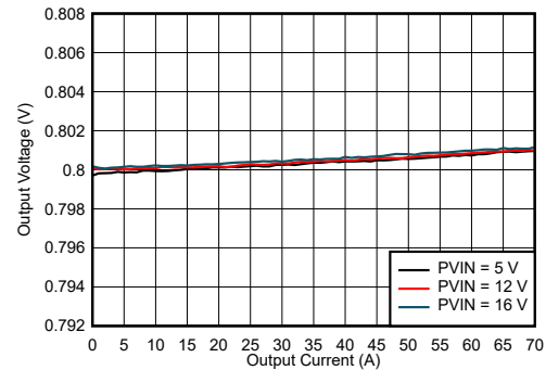
Figure 8-11. Load Regulation
