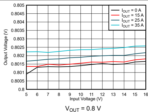
Figure 8-3. Line Regulation
