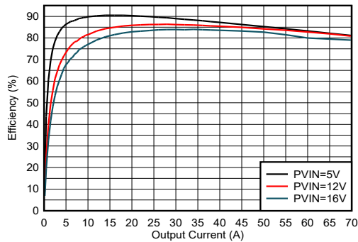
Figure 8-10. Efficiency vs Output Current
