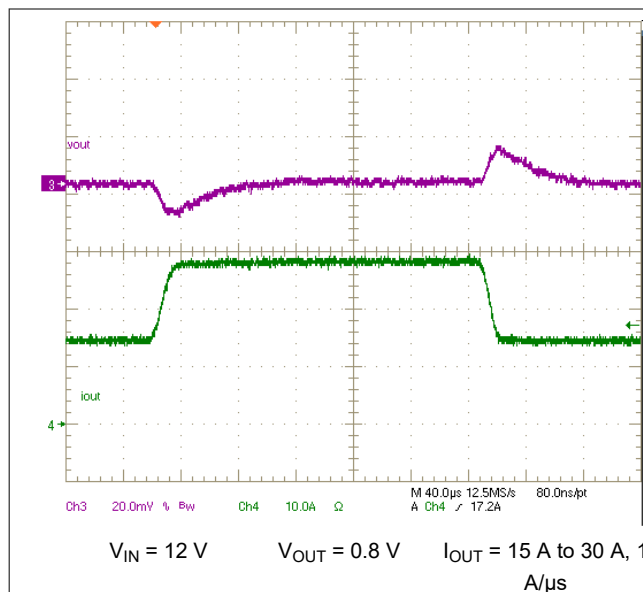
Figure 8-16. Load Transient Response
