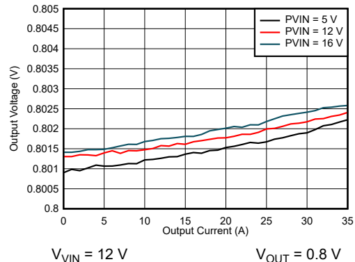
Figure 8-2. Load Regulation
