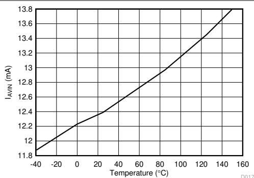
Figure 5-11. Nonswitching Input Current ( I_{AVIN} ) vs Junction Temperature
