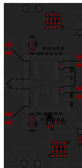
Figure 8-22. Bottom-Layer Layout (Top View)
