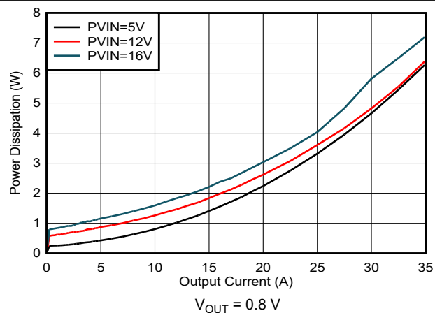
Figure 8-4. Power Dissipation
