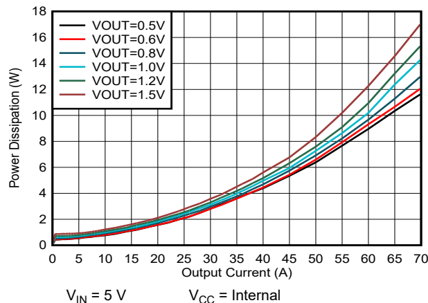
Figure 5-5. TPSM8D6C24 Power Dissipation vs Output Current
