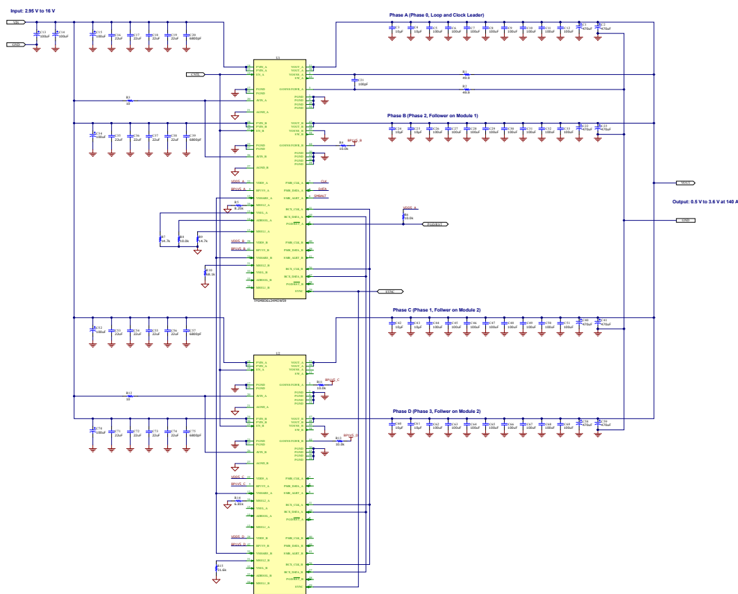
Figure 8-18. TPSM8D6C24 Four-Phase Application
