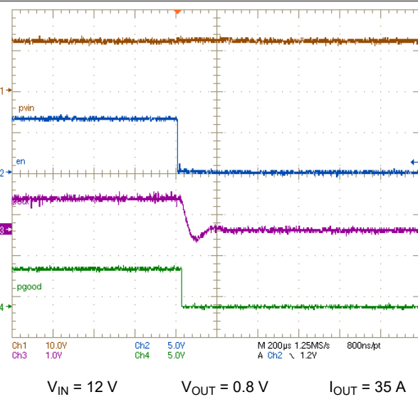
Figure 8-6. Shutdown from CNTL
