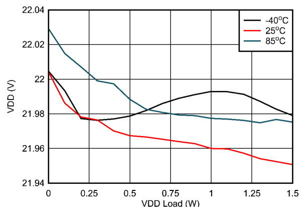
Figure 6-11. V_{D\overline{D}-VEE} Load Regulation: V_{IN} = 15V , V_{D\overline{D}-VEE} = 22V , V_{COM-VEE} = 4V
