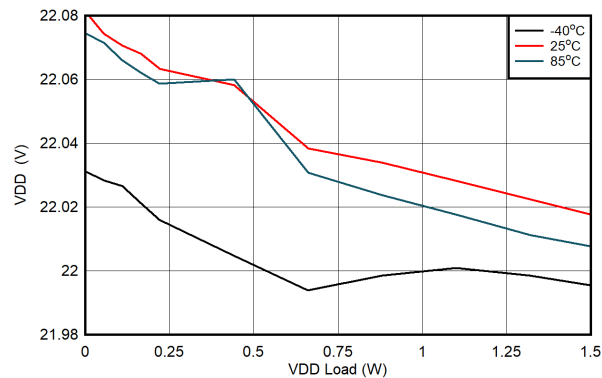
Figure 6-13. V_{D\overline{D}-VEE} Load Regulation: V_{IN} = 18V , V_{D\overline{D}-VEE} = 22V , V_{COM-VEE} = 4V
