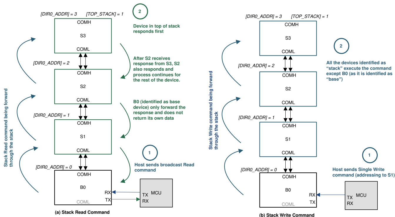
Figure 8-29. Stack Read/Write
