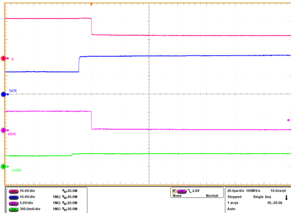
Figure 9-4. Zoom-In View of State Transition From LPM to Active Mode ( \overline{\text{LPM}} = Low, V_{\text{IN}} = 12V, \text{EN}/\text{UVLO} = High)
