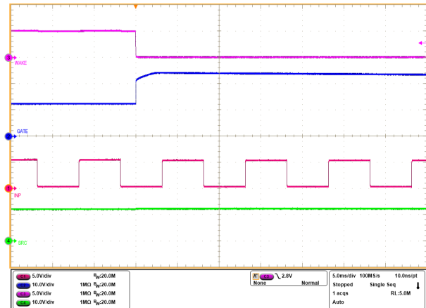
Figure 9-5. When \overline{\text{LPM}} = \text{Low} in LOAD WAKEUP state, INP Has No Control on GATE
