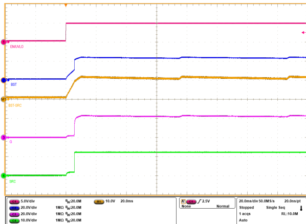
Figure 9-2. Start-Up Profile of Low Power Path (LPM = Low, VIN = 12V, No Load, C BST = 470nF)
