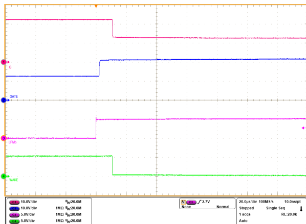
Figure 9-6. State Transition From LPM to Active Mode (LPM = Low to High, VIN = 12V, No Load)
