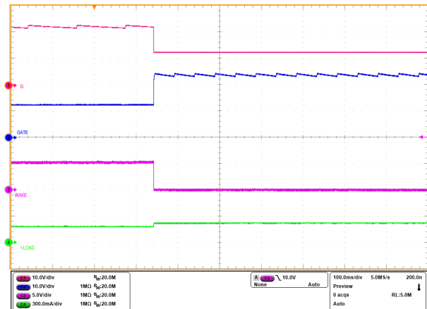
Figure 9-3. State Transition From LPM to Active Mode ( \overline{\text{LPM}} = Low, V_{\text{IN}} = 12V, \text{EN}/\text{UVLO} = High)
