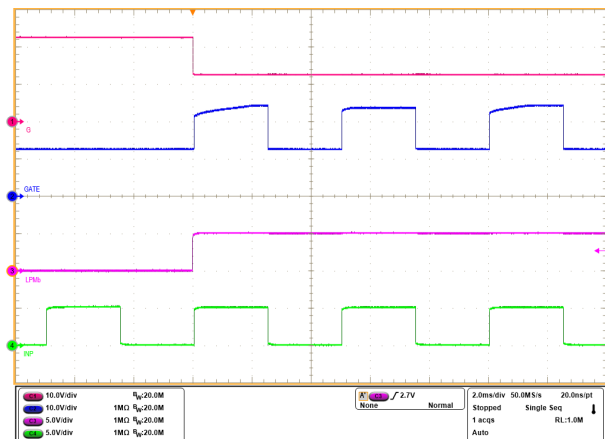
Figure 9-7. With \overline{\text{LPM}} = Low to High, INP Gained Control on GATE (VIN = 12V, No Load)
