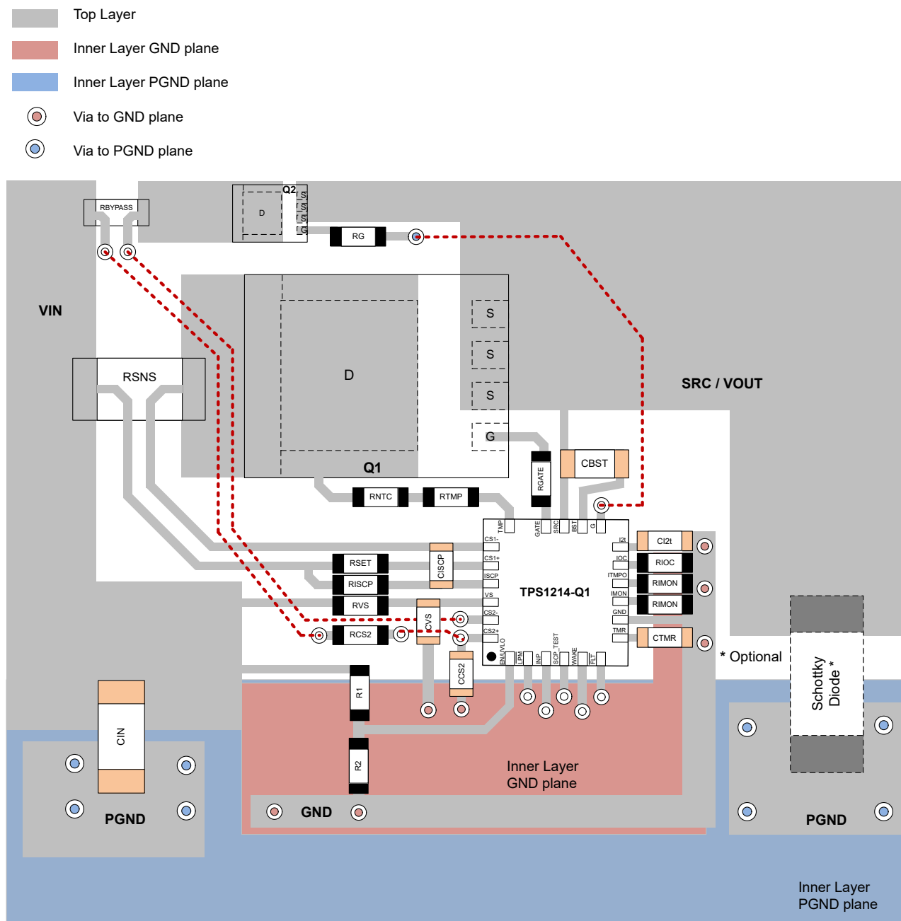
Figure 9-22. Typical PCB Layout Example of TPS1214-Q1
