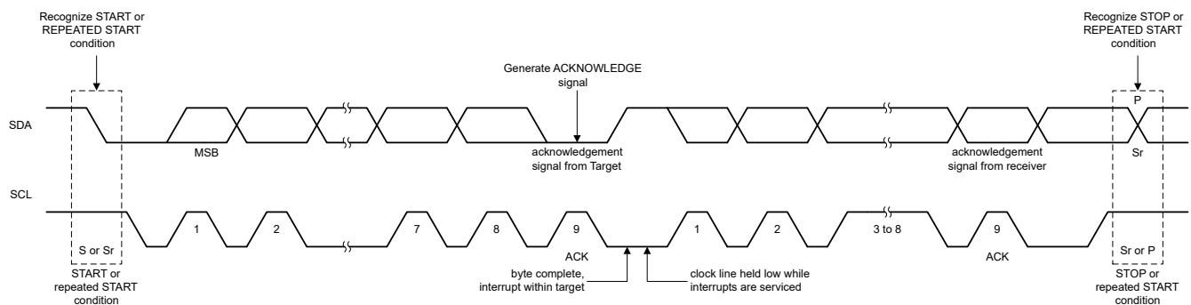
Figure 7-7. Bus Protocol
