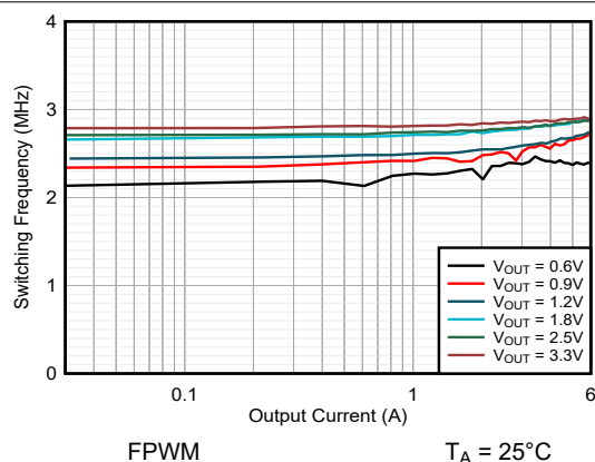
Figure 9-14. Switching Frequency V_{IN} = 5.0V
