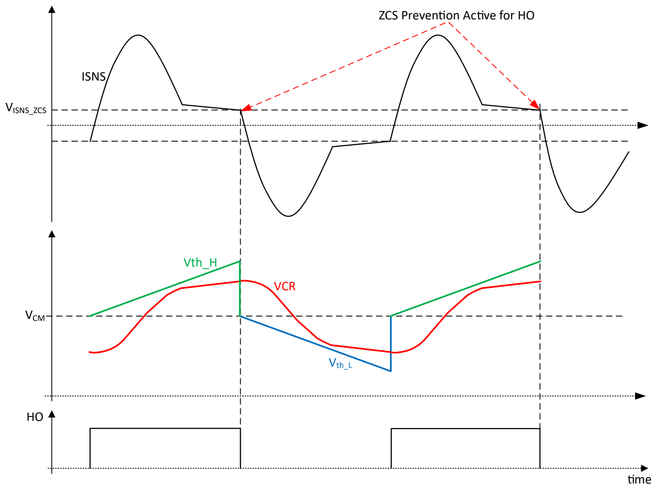
Figure 7-12. ZCS Protection
