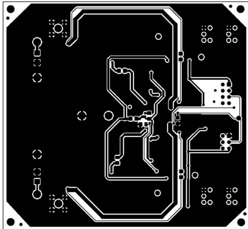
Figure 6-2. Bottom Assembly
