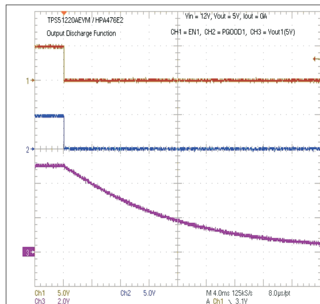
Figure 7-12. Enable Turn-Off With Discharge Waveform
