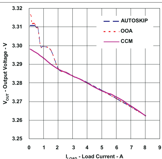
Figure 7-4. 12 V IN , 3.3-V Load Regulation
