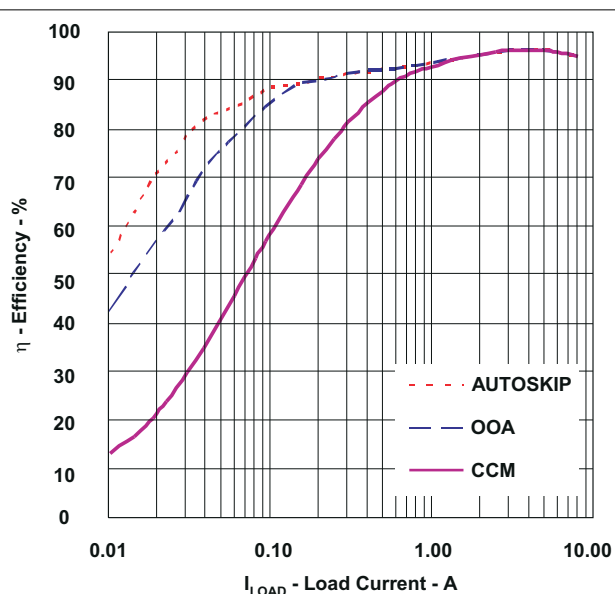
Figure 7-2. Efficiency, 12 V IN , 3.3-V Output
