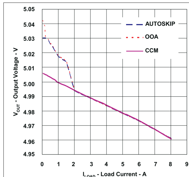
Figure 7-3. 12 V IN , 5.0-V Load Regulation
