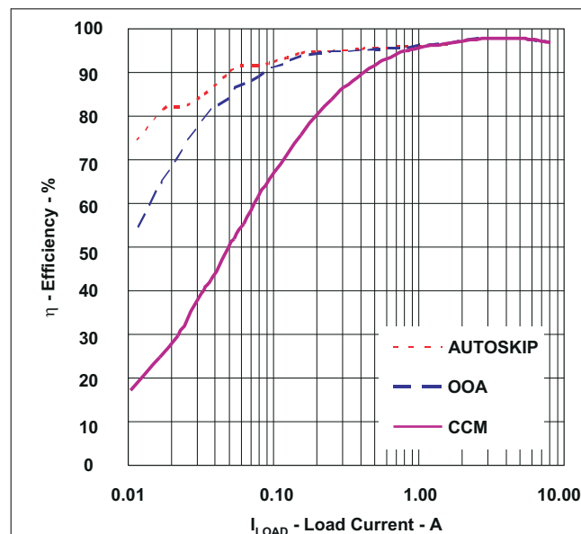
Figure 7-1. Efficiency, 12 V IN , 5.0-V Output
