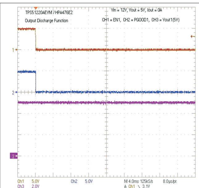
Figure 7-13. Enable Turn-Off Without Discharge Waveform
