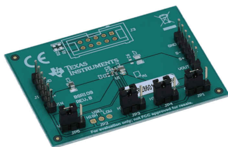
Figure 3-6. TPS628601EVM Angled View
